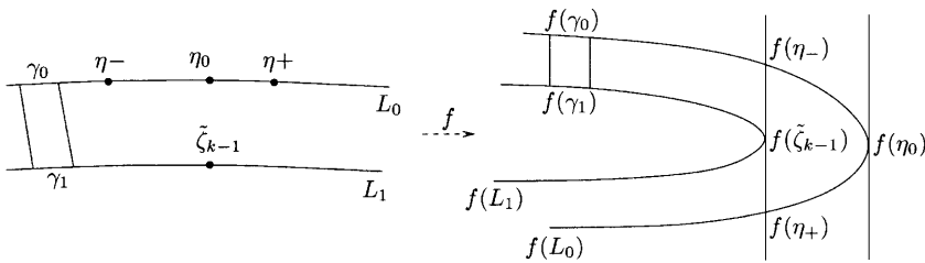
Fig. 3 Binding to a non-critical point
