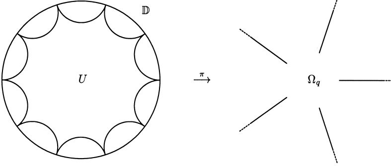
Fig. 4. The map \pi maps U to the slit plane \Omega_q
