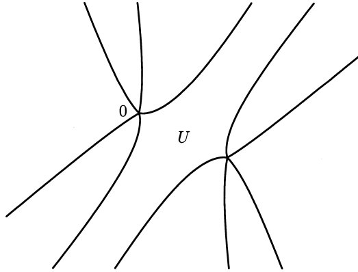
Fig. 2. Schematic example for q' = 5
