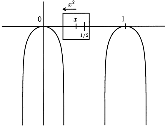
Fig. 3. The graph of the function f . The inequality f(x - x^2) < -x^2 means the lower left corner of the square is above the curve
