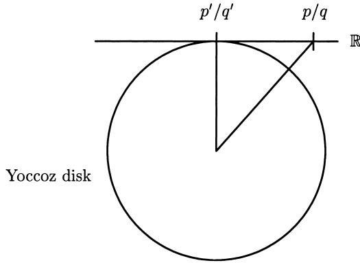
Fig. 1. The complex number \alpha lies somewhere in the Yoccoz disk
