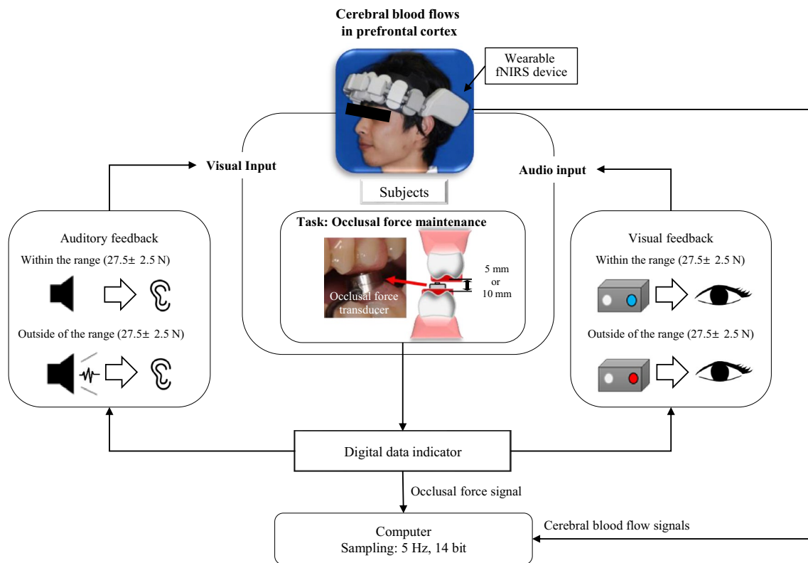
Fig. 1 Experimental configuration
