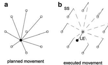
Fig. 2 a As shown in numerous studies, bidimensional movements are planned to follow a roughly straight line path ( continuous lines ) between the estimated hand initial location ( black circle ) and the target location ( white circles ). b The movements ( dashed lines ) are generated from the actual hand location ( white square ) leading to systematic end-point shifts (SS, continuous lines ). SS is the exact vectorial opposite of the localization error vector (LE) from the actual to the estimated hand initial location
