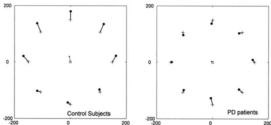
Fig. 4 Mean vector errors (thick continuous line) joining each target (crosses) to the corresponding movement end-point (large black dots). The systematic error averaged across targets is shown as a vector (thin continuous line) from the hand starting point
