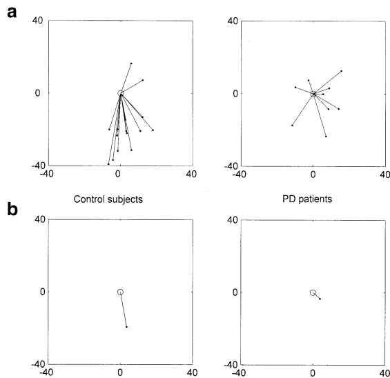
Fig. 5 a The mean bias in the estimation of the hand location, for each subject, as a vector ( continuous line ) originating from the starting position ( white circle ). b The mean bias in the estimation of the hand location averaged for all subjects. Left column displays data for the control subjects. Right column displays data for the PD patients. Axis scale is in millimeters
