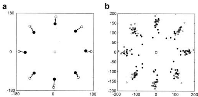
Fig. 6 a Mean movement end-point for the PD patients ( black circles ) and the control subjects ( white circles ). The movement starting point is represented by the central white square . The target location is represented by a black cross . Axis scale is in millimeters. b Mean movement end-point for each subjects. Same conventions as left panel
