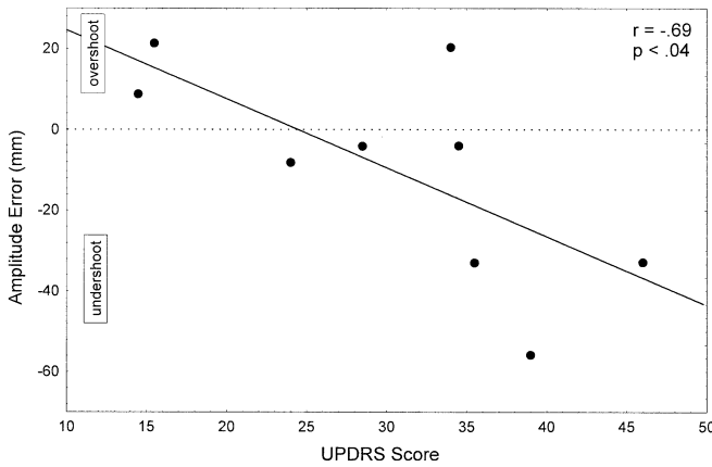
Fig. 7 Relationship between the mean amplitude error and the subject Unified Parkinson's Disease Rating Scale (UPDRS) score. The dashed line symbolize zero error. A point above this line indicates a target overshoot while a point below this line symbolizes a target undershoot. The significant correlation linking UPDRS scores and amplitude errors shows that the patients who presented with higher UPDRS score (i.e., a more severe stage of the disease) had a greater tendency to undershoot the target
