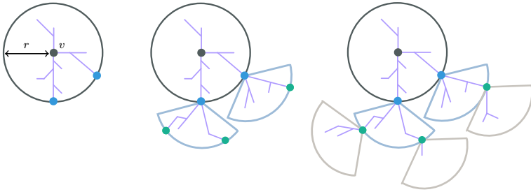
Fig. 1. Left: Upon exposing the localized FK-dynamics Z_T^v on B_r(v) , the connected component of v (purple) reaches two boundary points of B_r(v) (blue). Middle: The revealing procedure then exposes their localized configurations, in their balls of radius r . Right: The procedure continues in that manner until these connected components die out
