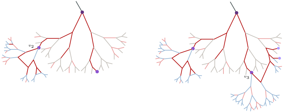
Fig. 3. Left: Proceeding from above, in the next generation, starting from v_2 \in \mathcal{V}_1 , reveal the edges of B_r^{out}(v_2) in \mathcal{G} ; in this case, this is not a tree, but is disjoint from \mathcal{A}_1 , so that \mathcal{A}_2 = B_r^{out}(v_2) . The configuration X_{\mathcal{A}_2,t}^1 is generated and concatenated with \tilde{\omega}_1 to form \tilde{\omega}_2 . Right: For v_3 \in \mathcal{V}_1 , B_r^{out}(v_3) is a tree, but it intersects \mathcal{A}_2 . As such, \mathcal{A}_3 = B_r^{out}(v_3) \setminus \mathcal{A}_2 . Running the FK-dynamics on \mathcal{A}_3 with all-wired boundary conditions ensures that X_{\mathcal{A}_3,t}^1 is nonetheless independent of the configuration we had revealed in \tilde{\omega}_2 . The light purple vertices are connected to \mathcal{V}_0 in \tilde{\omega}_3 and are added to \mathcal{V}_2 to form the next generation
