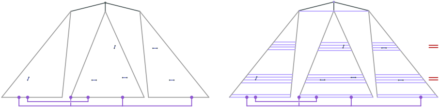
Fig. 5. Left: An L -Treelike ball with K -Sparse boundary conditions is depicted for L = K = 6 : the L edges that need to be removed to leave a tree are indicated in blue. Right: We modify the boundary conditions to be all wired (the wired component is depicted in purple) at one away from heights in \mathcal{Z} (marked by red dashes)
