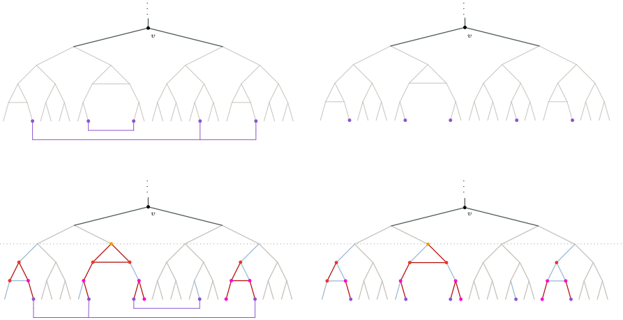
Fig. 4. Top: The ball B_R(v) for R = 5 , with a K -sparse boundary condition \tau for K = 4 (left), and the free boundary condition \xi = 0 (right). Bottom: The configurations revealed by the procedure of Definition 14, showing \mathcal{C}_{\mathfrak{N}}^{i_0}(\omega^\tau) (red, left) along with its outer edge boundary in \mathcal{Q}_{i_0} (light blue), revealing the dotted line (depth i_0 ) to be the largest i for which the set \mathcal{V}_i is a singleton. The vertices that would have been exposed for larger values of i are colored in different colors. The coupled edge configuration \omega^0(\mathcal{C}_{\mathfrak{N}}^{i_0}(\omega^\tau)) is depicted on the right (open edges in red, closed edges in blue). The exposed configurations on \mathcal{C}_{\mathfrak{N}}^{i_0}(\omega^\tau) induce free boundary conditions on E(B) \setminus \bar{\mathcal{C}}_{\mathfrak{N}}^{i_0}(\omega^\tau)
