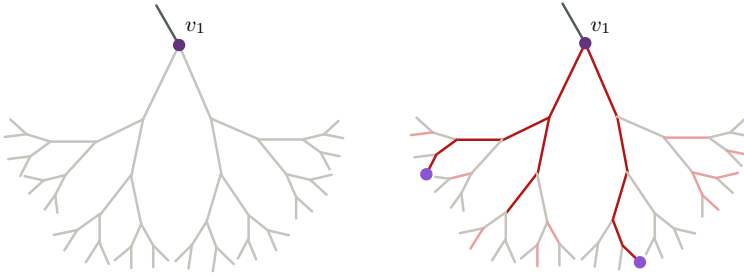
Fig. 2. Left: We initialize the process with r = 5 from \mathcal{V}_0 = \{v_1\} (dark purple) and incident edge \mathcal{A}_0 (black). The process begins by revealing A_1 = B_r^{out}(v_1) , depicted in gray. Right: The process then reveals the configuration X_{A_1,t}^1 , given by \kappa_{A_1,t} steps of FK-dynamics for \pi_{A_1}^1 , to form \tilde{\omega}_1 (open edges in red/pink). Vertices in \partial A_1 shown to be connected to v_1 in X_{A_1,t}^1(A_1) are added to \mathcal{V}_1 (purple)
