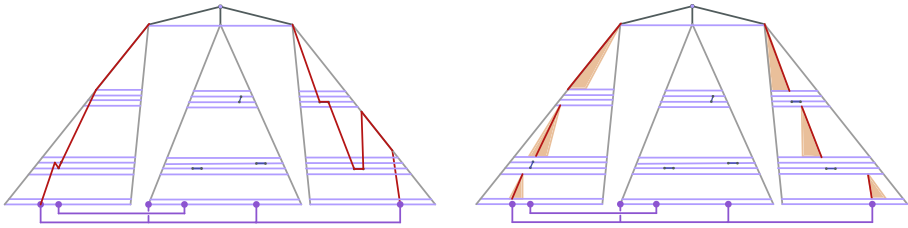
Fig. 6. Left: Two disjoint components (red) of the vertices in \mathfrak{B}_{B,\xi} , together intersect every depth in the ball and satisfy the event \Upsilon_{B,\xi} . Right: The two components contain corresponding sequences of open leaf-to-root paths (red) in independent wired subtrees (shaded, orange) whose endpoints are amongst the ancestors of vertices of H or \mathfrak{B}_{B,\xi}
