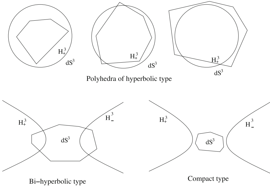
Fig. 5. Three types of polyhedra in HS^3
