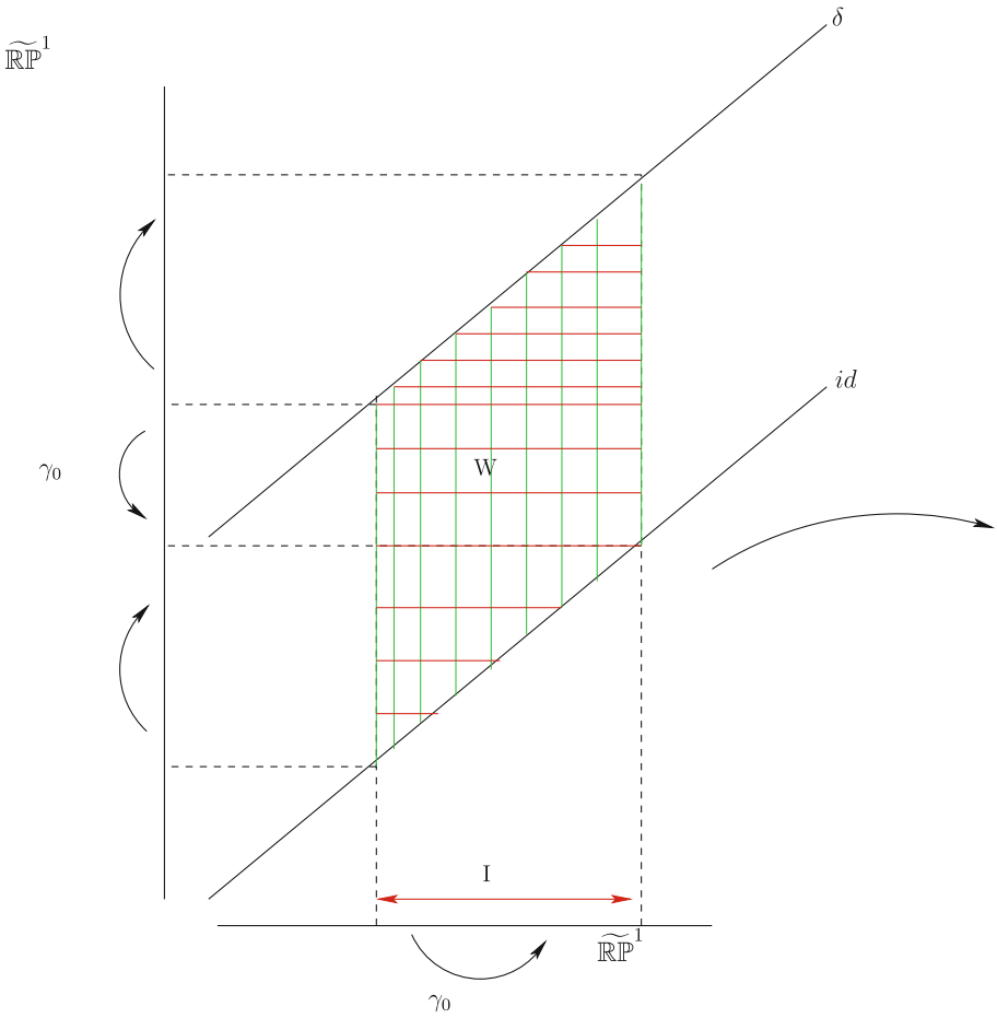
Fig. 9. The domain W and its quotient T'
