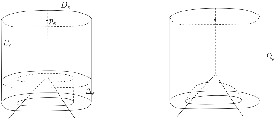
Fig. 11. Construction of a singular tube with an interaction of two particles
