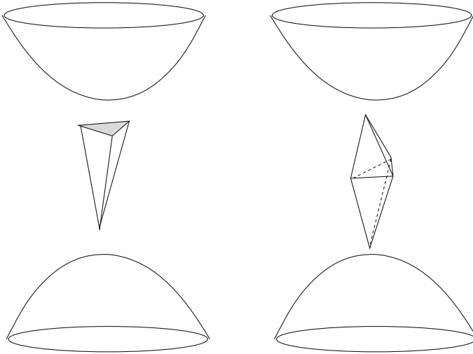
Fig. 7. Two polyhedra of compact type
