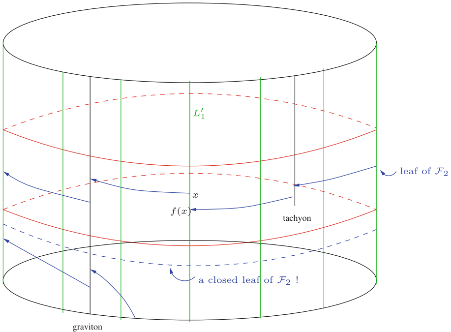
Fig. 10. First return maps. The identification maps along lines above time-like and light-like singularities compose the almost horizontal broken arcs which are contained in leaves of \mathcal{F}_2
