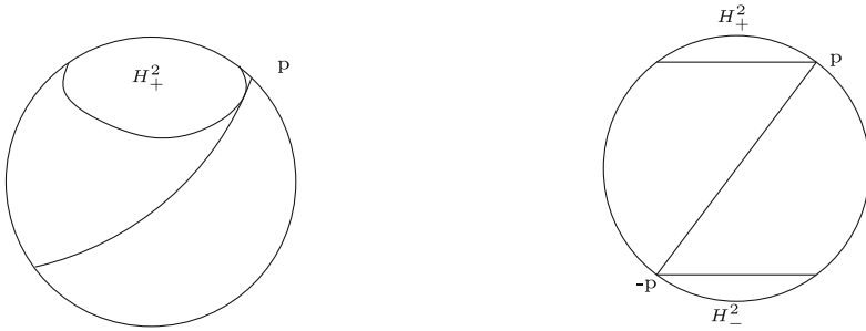
Fig. 1. A cuspidal singularity appears by taking the quotient of a half-sphere in HS^2 containing \mathbb{H}_+^2 and tangent to \partial\mathbb{H}_+^2 at a point p . The opposite point -p then corresponds to a past extreme BTZ-like singularity
