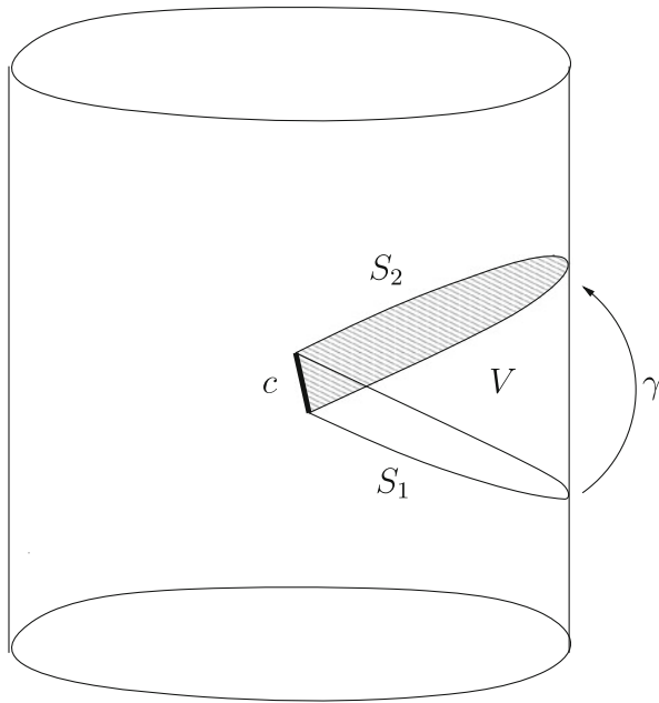
Fig. 3. The cylinder represents the boundary of the conformal model of AdS. If we remove the domain V and glue S_1 to S_2 we get a spacetime with one tachyon. If we keep V and glue S_1 to S_2 , we obtain a spacetime with one Misner singular line
