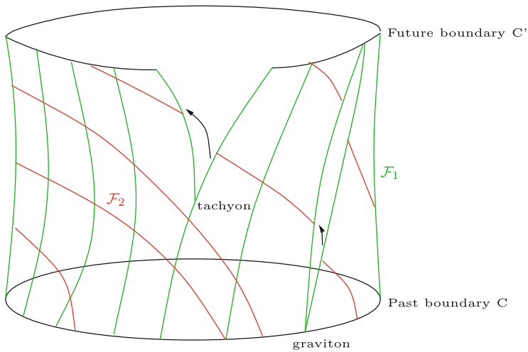
Fig. 8. Regularization of a tachyon and a light-like singularity
