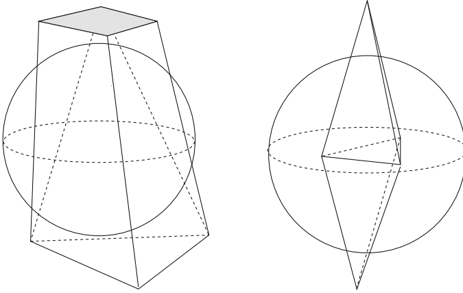
Fig. 6. Two polyhedra of hyperbolic type
