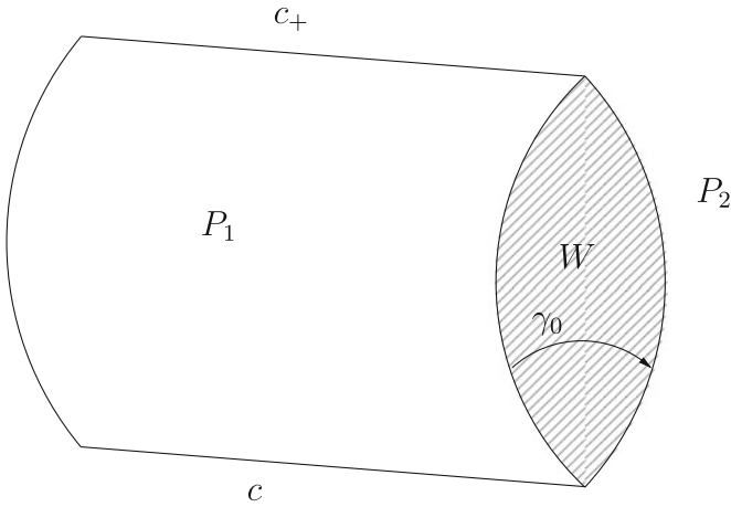
Fig. 2. By removing the domain W and glueing P_1 to P_2 one gets a spacetime with two tachyons. If we keep W and glue P_1 to P_2 , we obtain a spacetime with one future BTZ singular line and one past BTZ singular line
