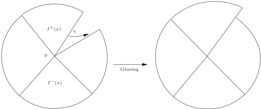
Fig. 4. Construction of a positive space-like singular line of degree 2
