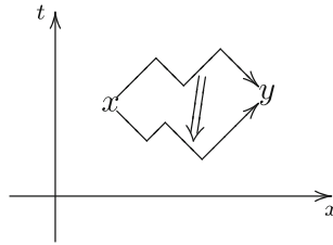
Fig. 4. A typical 2-morphism in P_2(\mathbb{R}^2)
