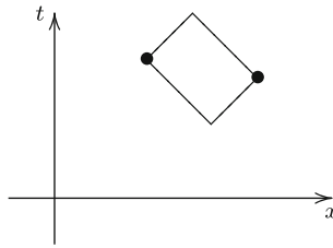
Fig. 1. A “causal subset” of 2-dimensional Minkowski space is the interior of a rectangle all of whose sides are lightlike. Such subsets are entirely fixed in particular by their left and right corners
