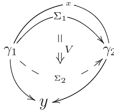
Fig. 8. A 3-morphism in a 3-path 3-category: a volume V , cobounding two surfaces \Sigma_1 and \Sigma_2 , which each cobound two paths \gamma_1 and \gamma_2 which each cobound two points x and y
