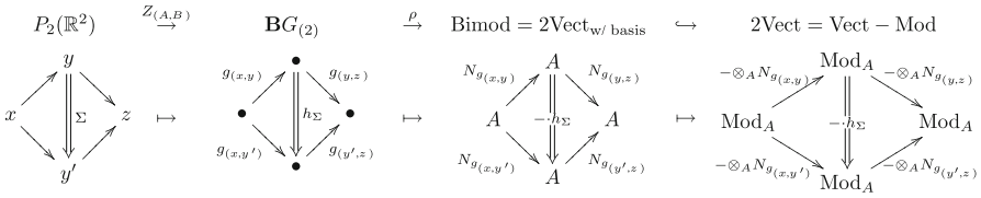
Fig. 6. 2-Vector transport coming from a 2-connection (A, B) \in \Omega^\bullet(\mathbb{R}^2, (\mathfrak{h} \rightarrow \mathfrak{g})) with values in the strict Lie 2-algebra (\mathfrak{h} \rightarrow \mathfrak{g}) and the canonical representation \rho of the corresponding strict Lie 2-group G(2) on 2-vector spaces. The 2-FQFT obtained this way assigns algebras to points, bimodules to paths and bimodule homomorphisms to surfaces. The corresponding local net \mathcal{A}_{Z(A,B)} assigns algebras of bimodule endomorphisms
