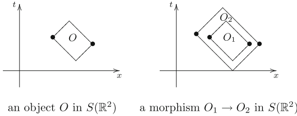
Fig. 2. The category S(\mathbb{R}^2) of causal subsets of 2-dimensional Minkowski space. Objects are causal subsets, morphisms are inclusions of these
