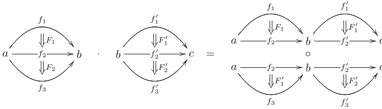
Fig. 5. The exchange law in 2-categories, which is the functoriality of horizontal composition on the Hom-categories, says that the 2-dimensional order of composition of 2-morphisms is irrelevant
