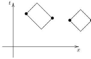
Fig. 3. Two spacelike separated causal subsets of \mathbb{R}^2
