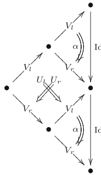
Fig. 7. The image under the boundary FQFT 2-functor Z_{\times}^{\leq} of a spacelike wedge on the left Minkowski half plane
