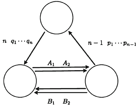
Fig. 4. The n q fields gives n marked points in the quiver, which generates the whole module, and the (n - 1) p fields will give (n - 1) relation via superpotential. The sheaves representing the nodes are to be determined
