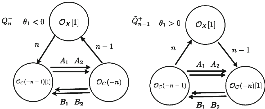
Fig. 8. The quiver Q_n^- and \tilde{Q}_{n-1}^+
