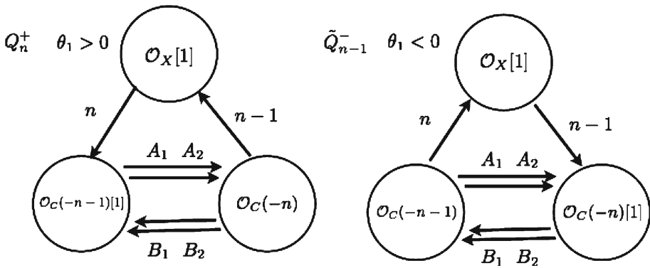
Fig. 7. The quiver Q_n^+ and \tilde{Q}_{n-1}^-
