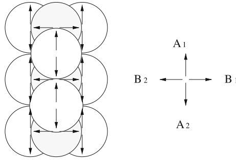
Fig. 3. This figure illustrates how to define a framed cyclic module from a pyramid partition
