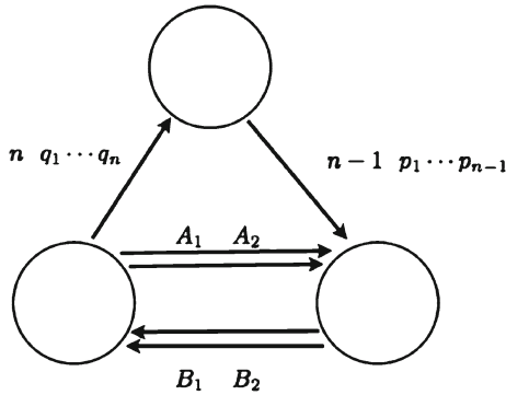
Fig. 5. This shows the arrow structure of the quiver \tilde{Q}_{n-1}
