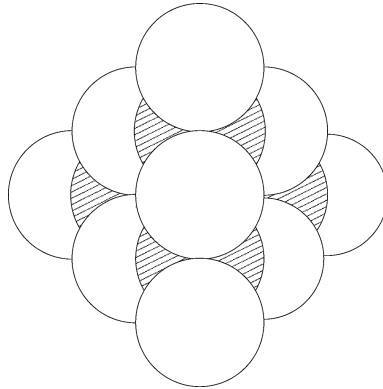
Fig. 2. This is the ERC for the finite type pyramid partition with length 3
