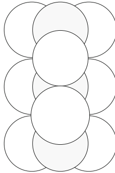
Fig. 1. This figure illustrates the length 2 ERC of the pyramid partition, from the zeroth layer to the 2nd layer
