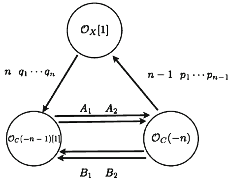
Fig. 6. The quiver diagram for the pyramid partition with length n ERC
