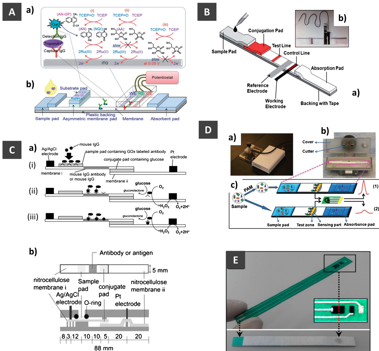
Fig. 4 Representative exemplary EC-LFAs with various electrode configuration integrated into LFS as well as assay platforms. A ITO electrode-coated glass plates assembled onto LFS (b) and detection principle (a), reprinted from [82] with permission from Royal Society of Chemistry. B The CNT conductive paper integrated immunostrip (a) and photograph of actual device adapted from [79] with permission from Royal Society of Chemistry. C The single-step quantitative EC-LFS
