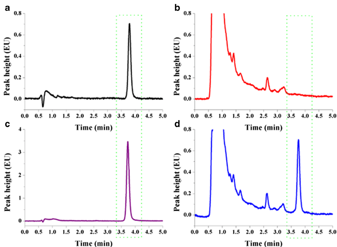
Fig. 4 Typical UHPLC–fluorescence chromatograms of (a) OTA standard solution (3 ng/mL), (b) blank ginger powder samples after cleanup by OS, (c) blank ginger powder samples spiked with OTA at the level of 15 µg/kg after cleanup by IS, and (d) after cleanup by OS (adapted from [35])
