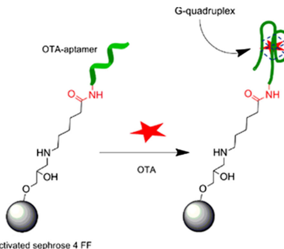
Fig. 2 Schematic presentation of the binding of OTA to aptamer (adapted from [35])
