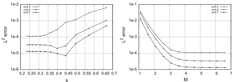
Fig. 3 The above figures report the L^2(D) -error behavior when D = (-1, 1) . The left one shows the error as a function of the quadrature spacing k for a fixed mesh size ( h = 1/8192 ) and domain truncation parameter ( M = 20 ). The right plot reports the error as a function of the domain truncation parameter M with fixed mesh size ( h = 1/8192 ) and quadrature spacing ( k = 0.2 ). The spatial error dominates when k is small (left) and M is large (right)
