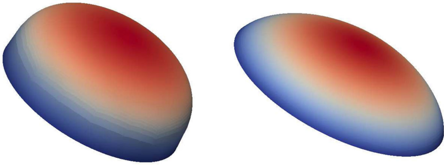
Fig. 4 Approximated solutions of (91) for s = 0.3 (left) and s = 0.7 (right) on the unit disk
