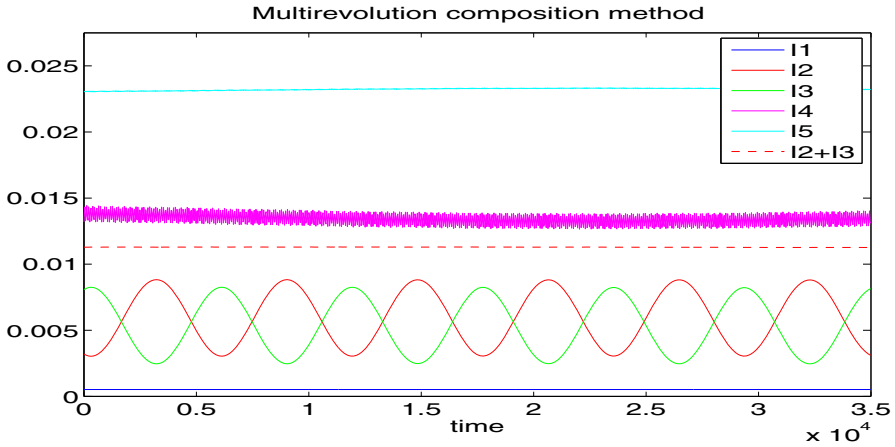
Fig. 7 (FPU, d = 2 ) energy exchanges, multirevolution composition method
