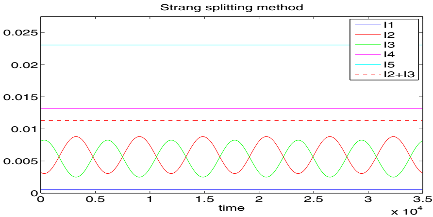
Fig. 6 (FPU, d = 2 ) energy exchanges, Strang splitting method
