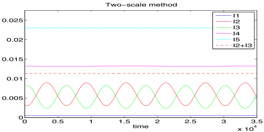
Fig. 8 (FPU, d = 2 ) energy exchanges, two-scale method
