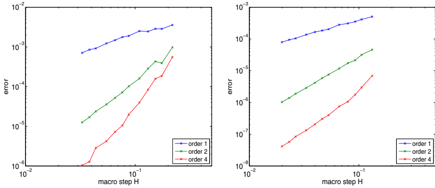
Fig. 4 (FPU, d = 1 ) error versus macrostep for \epsilon = 4 \times 10^{-5} (left) and \epsilon = 10^{-5} (right)
