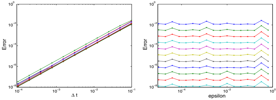
Fig. 5 (FPU, d = 1 ) left error as a function of \Delta t for \varepsilon = 2^N \times 10^{-2} , with N \in \{6, \dots, 1, 0, -1, \dots, -10\} . Right error as a function of \varepsilon for \Delta t = 2\pi/2^N with N \in \{6, \dots, 16\}
