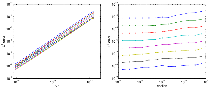
Fig. 12 Left L^2 error versus \Delta t for \epsilon = 2^N \times 10^{-2} , with N \in \{6, \dots, 1, 0, -1, \dots, -6\} . Right L^2 error versus \epsilon for \Delta t = 2\pi/2^N with N \in \{9, \dots, 16\}
