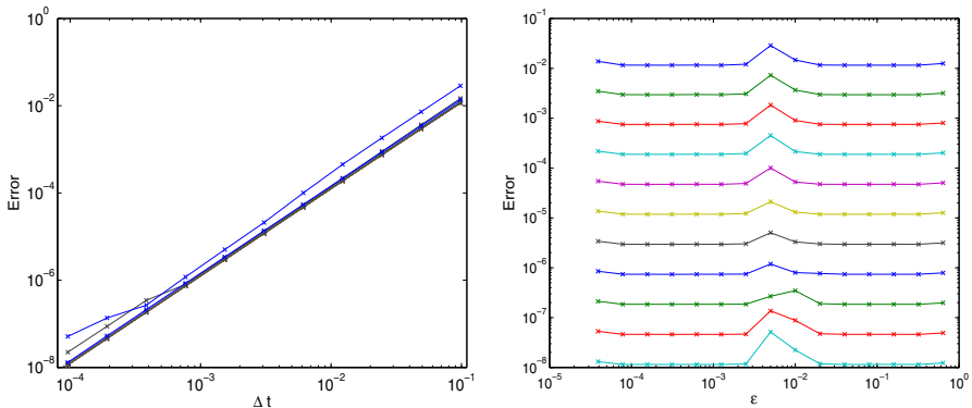
Fig. 9 (FPU, d = 1 ) Left error as a function of \Delta t for \varepsilon = 2^N \times 10^{-2} , with N \in \{6, \dots, 1, 0, -1, \dots, -10\} . Right error as a function of \varepsilon for \Delta t = 2\pi/2^N with N \in \{6, \dots, 16\}
