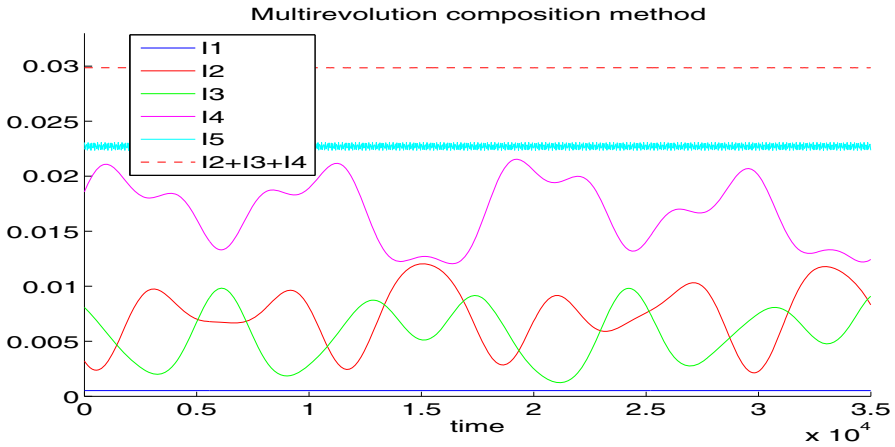
Fig. 2 (FPU, d = 1 ) energy exchanges, multirevolution composition method
