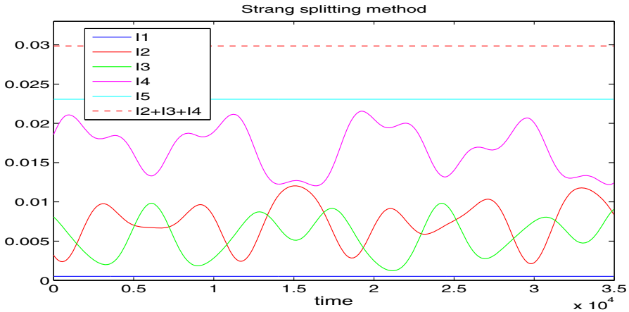
Fig. 1 (FPU, d = 1 ) energy exchanges, Strang splitting method
