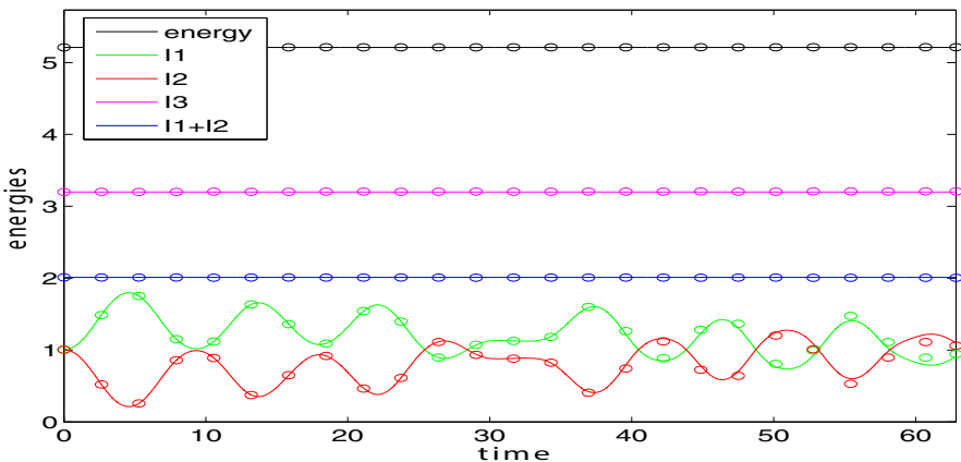
Fig. 10 Energy exchanges for \varepsilon = 0.0001 , computed with the Strang splitting method (plain lines) and the MRCM (circles) with N = 60
