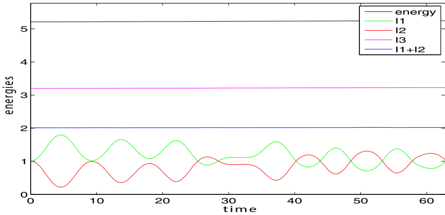
Fig. 11 Energy exchanges for \epsilon = 0.0001 , computed with the two-scale method
