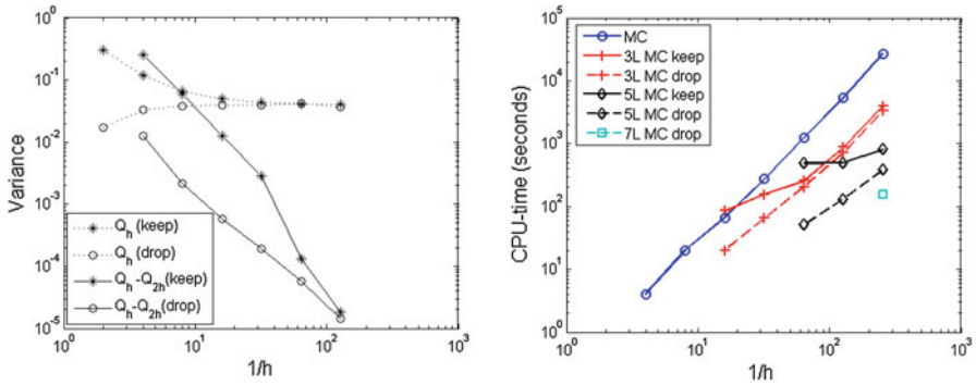
Fig. 4 Left Plot of \mathbb{V}[M_\omega^{(4)}(u_h)] and \mathbb{V}[M_\omega^{(4)}(u_h) - M_\omega^{(4)}(u_{2h})] , for (3.11) with d = 2, \lambda = 0.1, \sigma^2 = 1, \psi = x_1, K_\ell = 4h_\ell^{-1}, h^* = 1/256 and K^* = 1,024 . Right Plot of cost CPU-time versus 1/h for a fixed tolerance of the sampling error of \delta = 10^{-3} , for the same model problem
