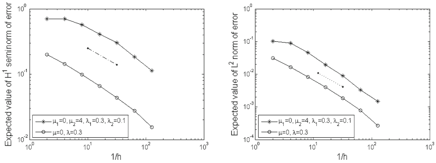
Fig. 5 Left Plot of \mathbb{E}[|u_{h^*} - u_h|_{H^1(D)}] versus 1/h for model problem (3.11) with 2-norm exponential covariance, with \mu = \mu_1 = 0, \mu_2 = 4, \lambda = \lambda_1 = 0.3, \lambda_2 = 0.1, \sigma^2 = \sigma_1^2 = \sigma_2^2 = 1 and h^* = 1/256 . Right Plot of \mathbb{E}[\|u_{h^*} - u_h\|_{L^2(D)}] . The gradient of the dash-dotted (resp. dotted) line is -1/2 (resp. -1 )
