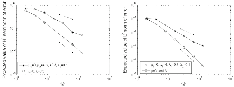
Fig. 6 Left Plot of \mathbb{E}[|u_{h^*} - u_h|_{H^1(D)}] versus 1/h for model problem (3.11) with Gaussian covariance, with \mu = \mu_1 = 0, \mu_2 = 4, \lambda = \lambda_1 = 0.3, \lambda_2 = 0.1, \sigma^2 = \sigma_1^2 = \sigma_2^2 = 1, h^* = 1/256 and K^* = 170 . Right Plot of \mathbb{E}[\|u_{h^*} - u_h\|_{L^2(D)}] . The gradient of the dash-dotted (resp. dotted and dashed) line is -1/2 (resp. -1 and -2 )
