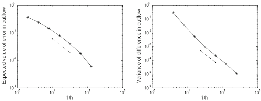
Fig. 2 Left Plot of |\mathbb{E}[M_\omega^{(4)}(u_{h^*}) - M_\omega^{(4)}(u_h)]| , for 2D model (3.11) problem with \lambda = 0.3, \sigma^2 = 1, \psi = x_1 and h^* = 1/256 . Right Corresponding variance \mathbb{V}[M_\omega^{(4)}(u_h) - M_\omega^{(4)}(u_{2h})] . The gradient of the dotted (resp. dashed) line is -1 (resp. -2 )
