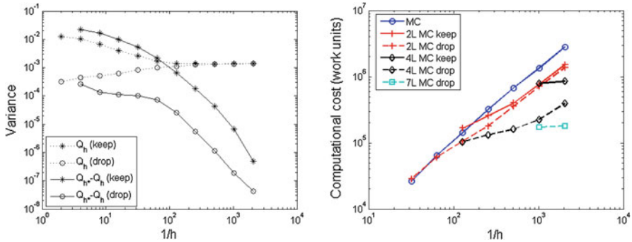
Fig. 3 Left Plot of \mathbb{V}[M^{(1)}(u_h)] and \mathbb{V}[M^{(1)}(u_h) - M^{(1)}(u_{2h})] , for (3.10) with d = 1, \lambda = 0.01, \sigma^2 = 1, K_\ell = h_\ell^{-1}, h^* = 1/4096, K^* = 4,096 and x^* = 2,049/4,096 . Right Plot of cost versus 1/h for a fixed tolerance of the sampling error of \delta = 10^{-3} , for the same model problem
