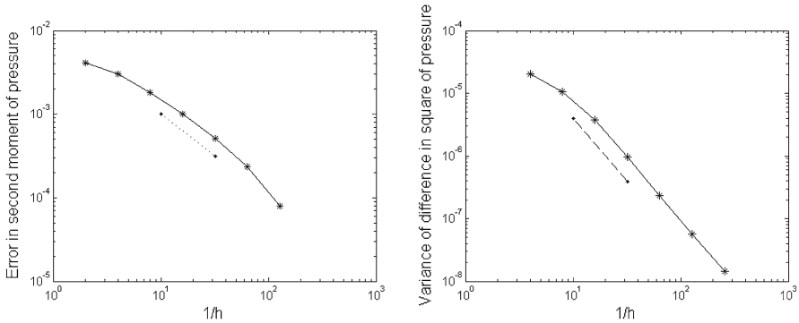
Fig. 1 Left plot |\mathbb{E}[M^{(2)}(u_{h^*})^2 - M^{(2)}(u_h)^2]| for 2D model problem (3.10) with \lambda = 0.3, \sigma^2 = 1 and h^* = 1/256 . Right plot Corresponding variance \mathbb{V}[M^{(2)}(u_h)^2 - M^{(2)}(u_{2h})^2] . The gradient of the dotted (resp. dashed) line is -1 (resp. -2 ).
