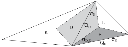
Fig. 1 Triangles K, L \in \mathcal{T}_h and dual volumes D, E \in \mathcal{D}_h associated with edges \sigma_D, \sigma_E \in \mathcal{E}_h
