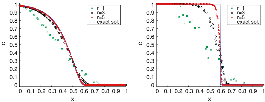
Fig. 5 Solution profiles for y = 0.5 at t = 0.5 , \delta = 0.05 (left) and \delta = 0.0001 (right)
