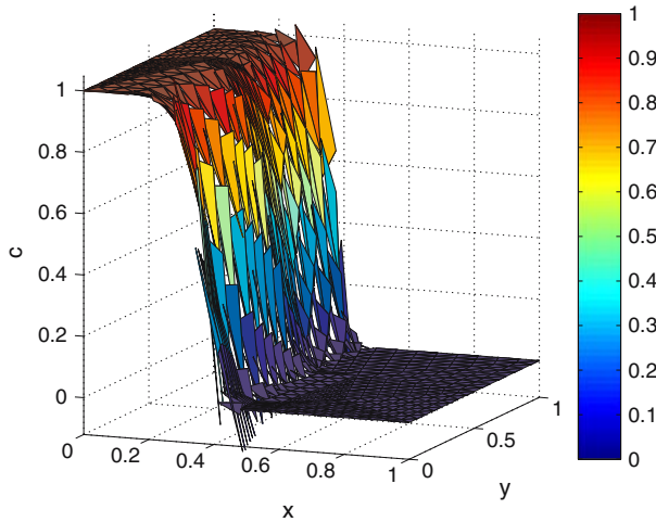
Fig. 3 Approximate solution at t = 0.25, \delta = 0.01, r = 3
