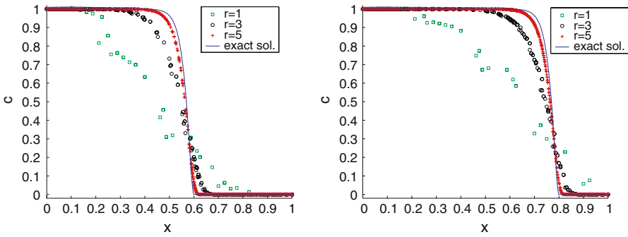
Fig. 4 Solution profiles for y = 0.5 and \delta = 0.01 , at t = 0.5 (left) and at t = 0.75 (right)
