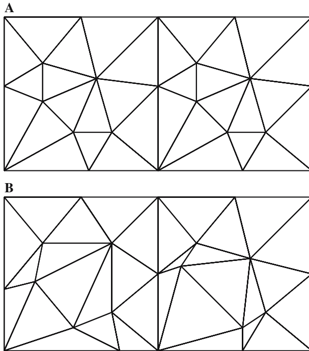
Fig. 6 Initial meshes A (top) and B (bottom)
