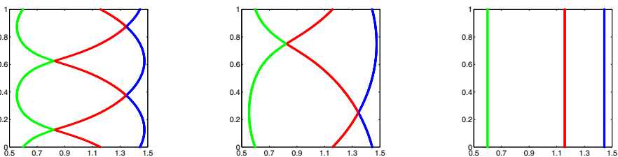
Fig. 5 The norms of the roots of f along the paths \eta_1, \eta_2 and \gamma (from left to right). The vertical axis is k , the horizontal axis represents the norms of particular roots
