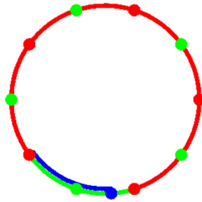
Fig. 7 Situation for s + t = 5 and \arg(q) = 0 . For a fixed \arg(q) , the set \widehat{U}_j^A is the union of s + t open segments between the red (dark) points (one is exemplarily depicted in green (light) color here). Each of the segments is retracted to their green (light) midpoint under \widehat{F} . For a point \arg(p) (the blue (very dark) point here), the corresponding value \arg(p) \bmod \frac{2\pi}{s+t} is the length of the blue (very dark) segment. Thus, indeed, \widehat{F}(\widehat{U}_j^A, 1) = \rho_{(\pi/(s+t), 0)} (color figure online)
