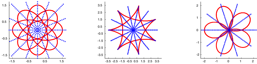
Fig. 3 Three hypotrochoids: The trajectory of the fiber functions f^1 - p , g^1 - p and h^1 - p for the norm v = 1 and trinomials f = z^8 + pz^3 + 0.5 , g = z^7 + pz^2 + 2.5 and h = z^5 + pz + 1 with their corresponding union of rays F(s, t, q) (the blue dotted rays). The hypotrochoids and F(s, t, q) are located in a complex plane, which is a \mathbb{C} -slice of the parameter space \tilde{T}_A (color figure online)
