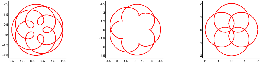
Fig. 4 Epitrochoids for (R, r, d) = (15/16, 9/16, 1), (5/2, 1, 1) and (4/5, 1/5, 1) in the complex plane. As we have r = d in the second example, we see that the epitrochochoid in fact is an epicycloid
