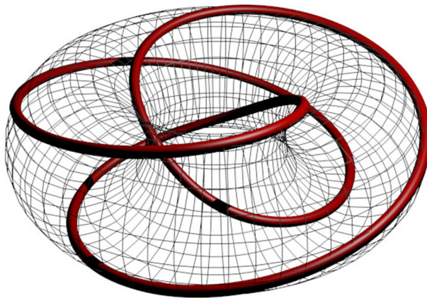
Fig. 6 The curve \rho(0, 0) for s = 2 and s + t = 3 on a torus. By Corollary 5.4 it corresponds to the K(3, 2) —the trefoil knot
