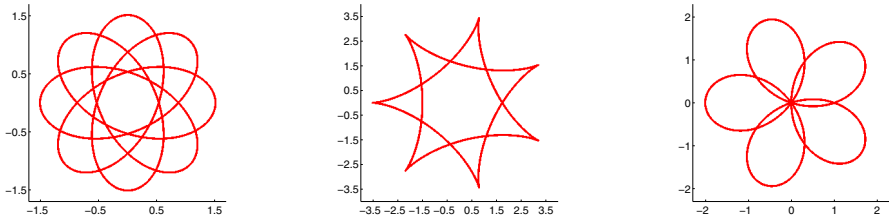
Fig. 1 Hypocycloids for (R, r, d) = (8/3, 5/3, 1/2), (7/2, 5/2, 5/2) and (5, 4, 1) . The second curve is a hypocycloid and the third one is a rhodonea curve, which are both special instances of hypocycloids
