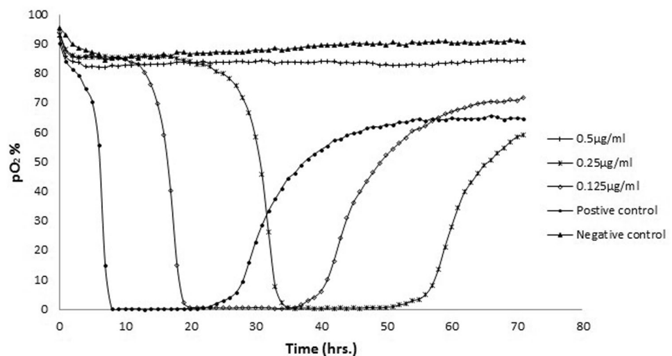
Fig. 2 The MBC of tobramycin against PAO1. The oxygen consumption of an overnight culture of planktonic cells of PAO1 treated with tobramycin using a fluorescent plate reader incubated at 30 °C for 72 h. The MBC represents the time to detect the lowest concentration that induced an increase in the oxygen concentration as a result of oxygen diffusion back into the wells following cell death. In contrast to the untreated positive control sample, the negative control represents an overnight culture injected with solution of sodium hypochlorite (10% v/v)
