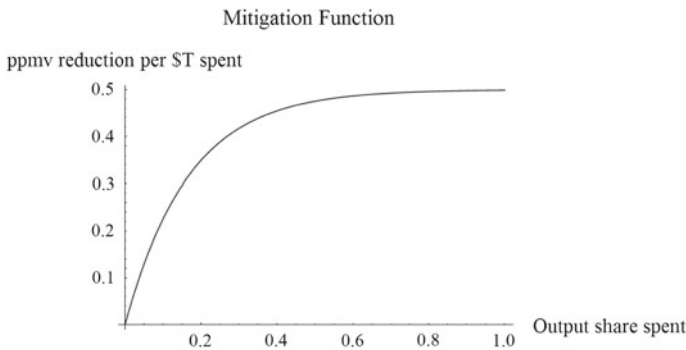
Fig. 2 Mitigation function for \zeta = 3 and \nu = 6
