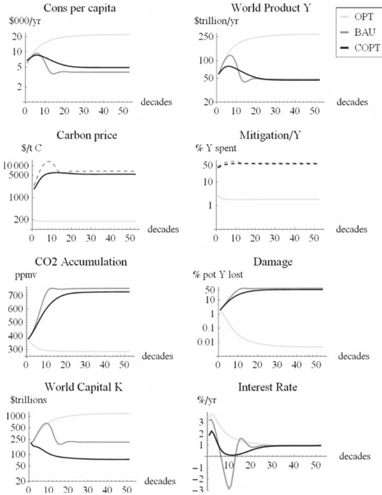
Fig. 3 The optimal equilibrium path, OPT, is plotted in pale gray , the BAU equilibrium in gray , and the constrained equilibrium, COPT, in dark gray . The carbon price on the optimal path is about $200/t, and the damage on the optimal path is less than 1% of potential output. The carbon price is the social marginal value of foregoing the emissions from 1t of carbon. For OPT and COPT, the carbon price is effective in economic decisions, but not in BAU (and is plotted as a dashed line ). For OPT, the mitigation percentage is the proportion of world product devoted to mitigation. For COPT and BAU, the mitigation percentage is the investment called for by the imputed carbon price (and is plotted as a dashed line ), while the actual mitigation is zero
