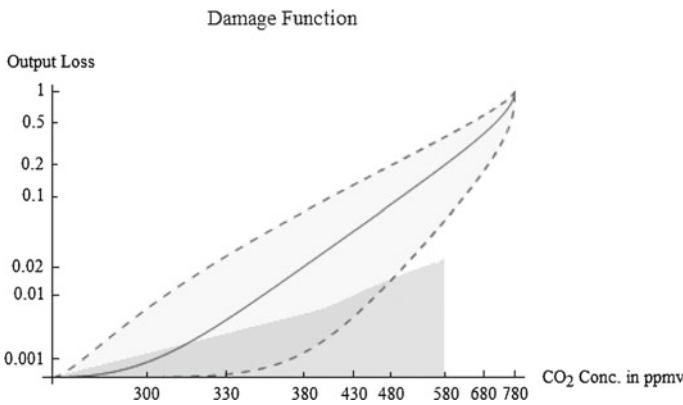
Fig. 1 Damage function with \gamma = 0.5
