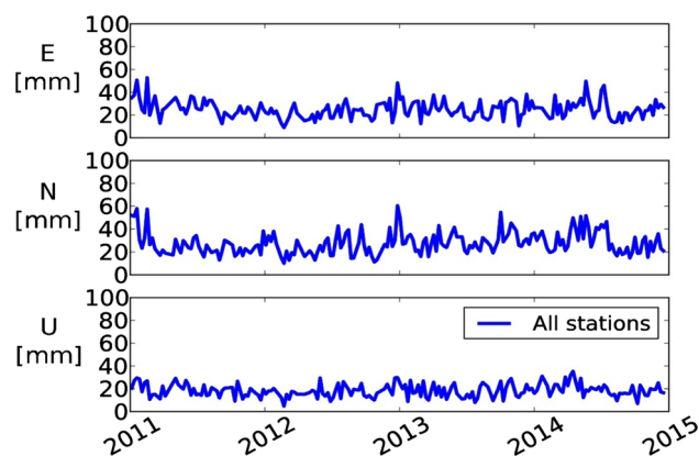
Fig. 4 WRMSs of station position residuals resulting from 7-parameter similarity comparisons between 9-day estimates based on SLR observations to GNSS satellites and the weekly ILRS official contribution to the computation of the ITRF2014
