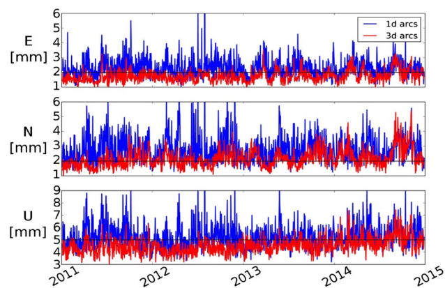
Fig. 2 WRMSs of station position residuals resulting from 7-parameter similarity comparisons between our daily (blue line) and 3-day (red line) GNSS solutions and the IGS repro2 combined results. The horizontal black lines indicate the upper limit of the general agreement shown by the solutions provided by the official IGS ACs
