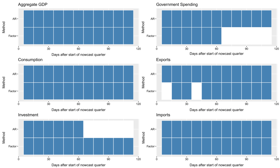
Fig. 5 Horizon MCS results—MSFE loss
