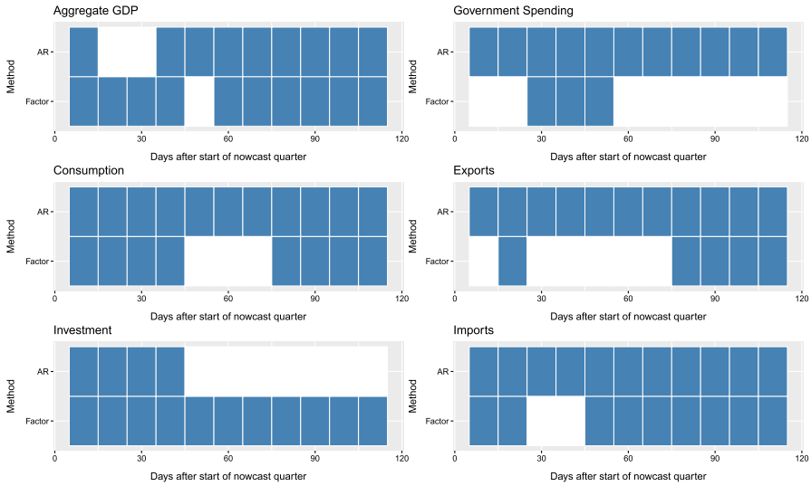
Fig. 7 Independent horizons MCS results—MSFE loss
