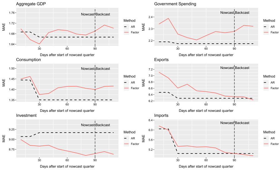
Fig. 2 MAE by nowcast horizon—GDP subcomponents
