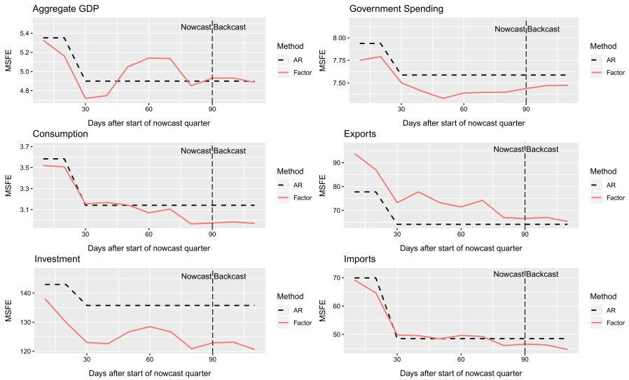
Fig. 10 MSFE by nowcast horizon—recursive
