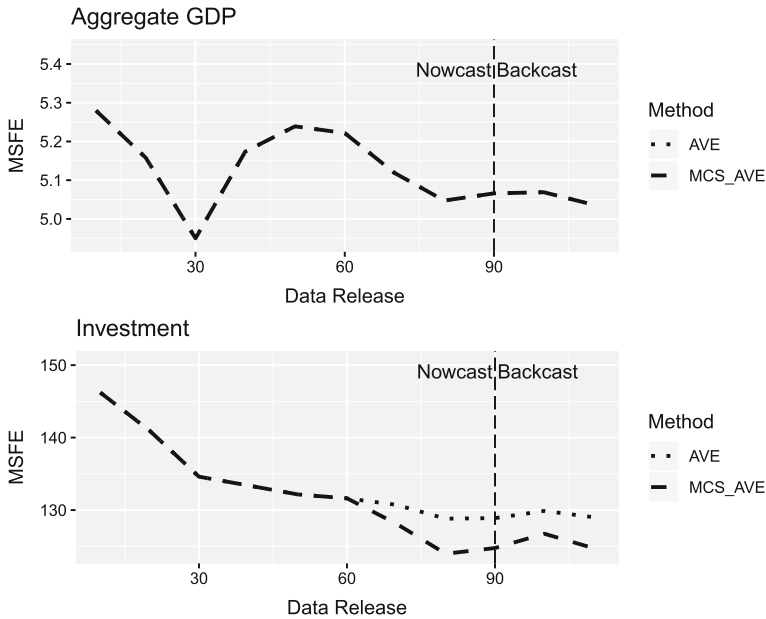
Fig. 8 MSFE of the nowcast combination
