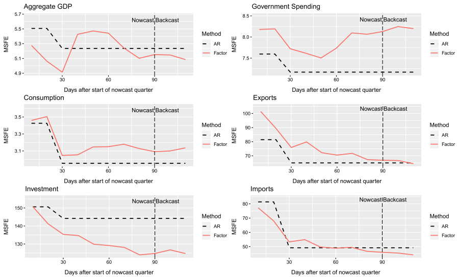
Fig. 3 MSFE by nowcast horizon—GDP subcomponents
