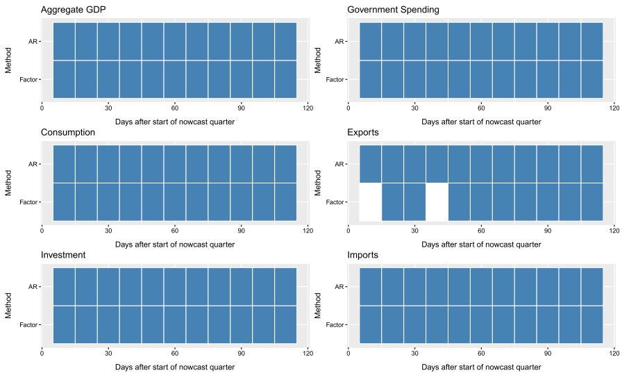
Fig. 12 Horizon MCS results—recursive—MSFE loss
