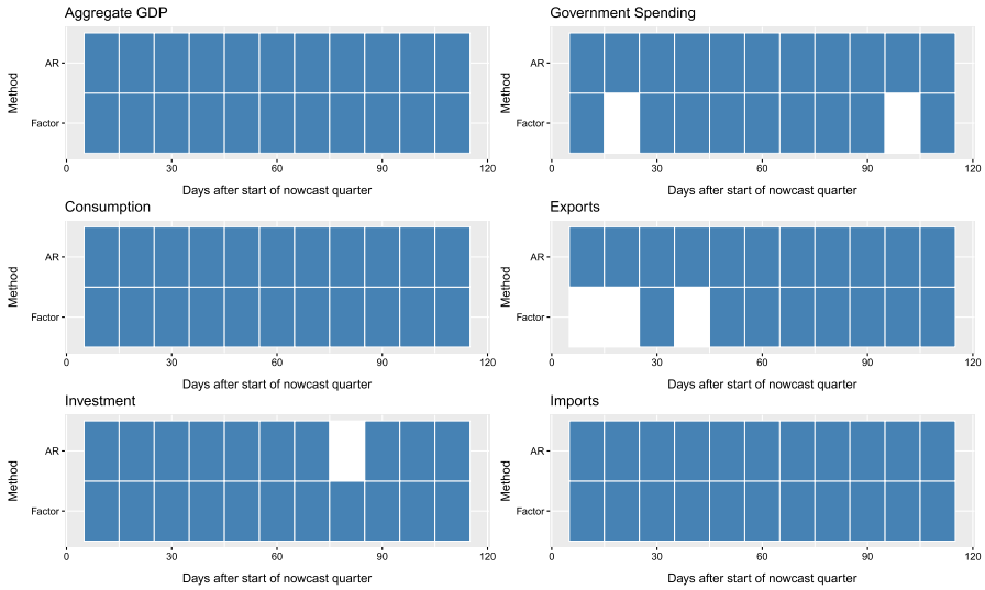
Fig. 4 Horizon MCS results—MAE loss
