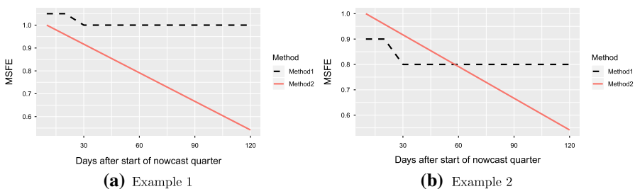
Fig. 1 Illustrative example of MSFE
