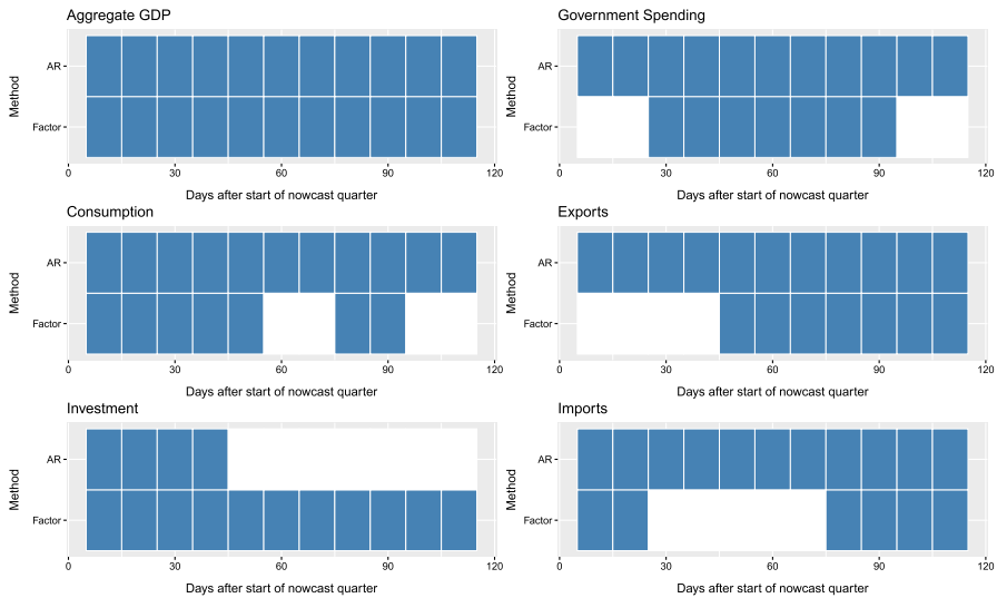
Fig. 6 Independent horizons MCS results—MAE loss
