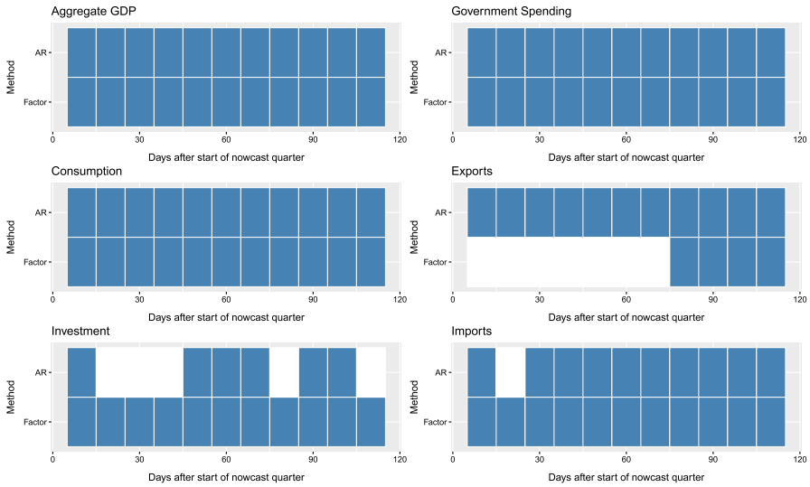
Fig. 11 Horizon MCS results—recursive—MAE loss
