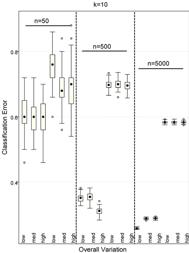
Fig. 5 Classification (prediction) error for all Bayesian network models, for k = 10 folds, for three case file sizes n . Boxplots correspond to 100 replications for each model. In each set of 6 boxplots, the first three are for Bayesian network models with high model variable dependency, and the second three are for Bayesian network models with low variable dependency
