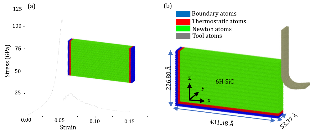
Fig. 7 a Molecular dynamics model for uniaxial compression and stress-strain curves from MD simulations, and b the nanocutting MD simulation model
