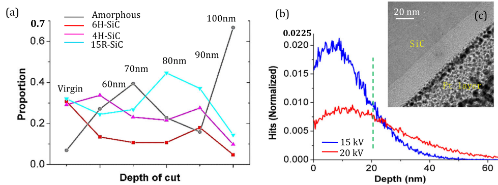
Fig. 5 a Proportion of SiC crystal structure changed with different depths of cut based on the EBSD (20 kV, 2.4 nA) data. b Penetration depth of the backscattered electrons with 15 kV and 20 kV (Casino simulation: SiC
