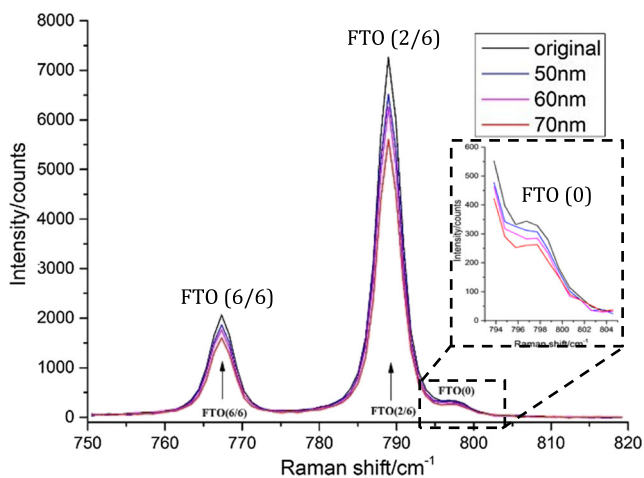
Fig. 6 Raman spectra of ductile removal surface for undeformed chip thicknesses of 50, 60, and 70 nm and unmachined surface
