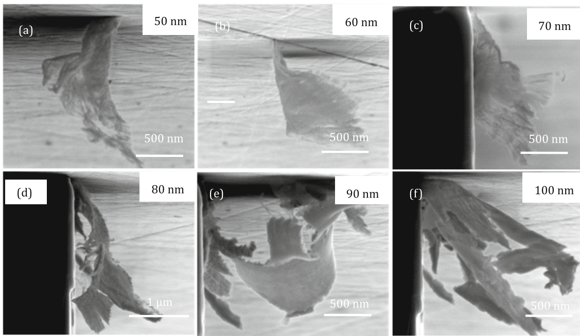
Fig. 3 SEM photographs of nanocutting chip morphology for different undeformed chip thicknesses
