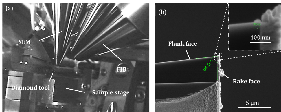
Fig. 1 Experimental setup of the nanometric cutting: a setup inside the vacuum chamber of SEM/FIB, b morphology of the diamond cutting tool
