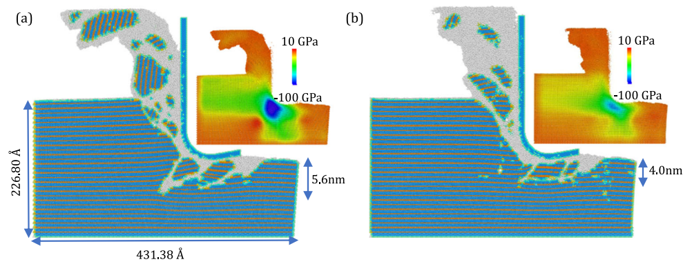
Fig. 14 Snapshots from the nanometric cutting simulations with 10 nm depth of cut by a normal nanocutting and b ion implant-assisted nanocutting. The upper right corner is the hydrostatic pressure distribution at the corresponding time
