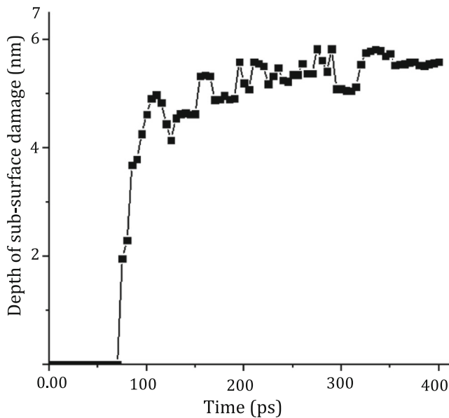
Fig. 15 Curve of subsurface damage depth with time under normal nanocutting
