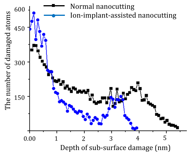
Fig. 16 Distribution of damaged atoms in the direction of subsurface damage depth
