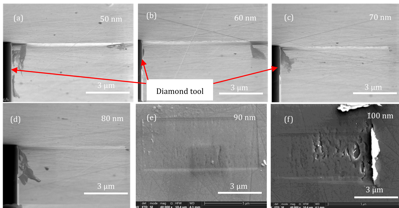
Fig. 2 SEM photographs of nanocutting surface morphology for different undeformed chip thicknesses
