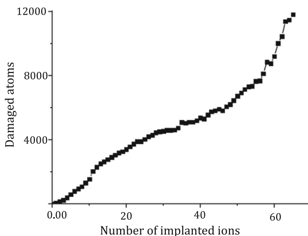
Fig. 12 Curve of damage atom with ion implantation
