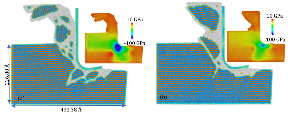
Fig. 8 Snapshots from the different nanometric cutting simulations. The upper right corner is the hydrostatic pressure distribution at the corresponding time. a Normal nanocutting with 10 nm depth of cut. b Stress-assisted nanocutting with 10 nm depth of cut under a 5.8 GPa uniaxial compression stress
