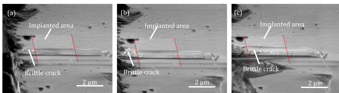
Fig. 18 The ion-implant-assisted 6H-SiC nanocutting results for continuous three times 90 nm depth of cut: a the first time, b the second time, c and the third time. The red dot lines show the boundary for ion implant area along the cutting direction
