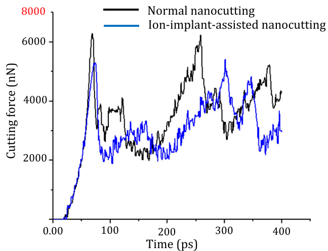
Fig. 17 Cutting force during nanometric cutting of 6H-SiC
