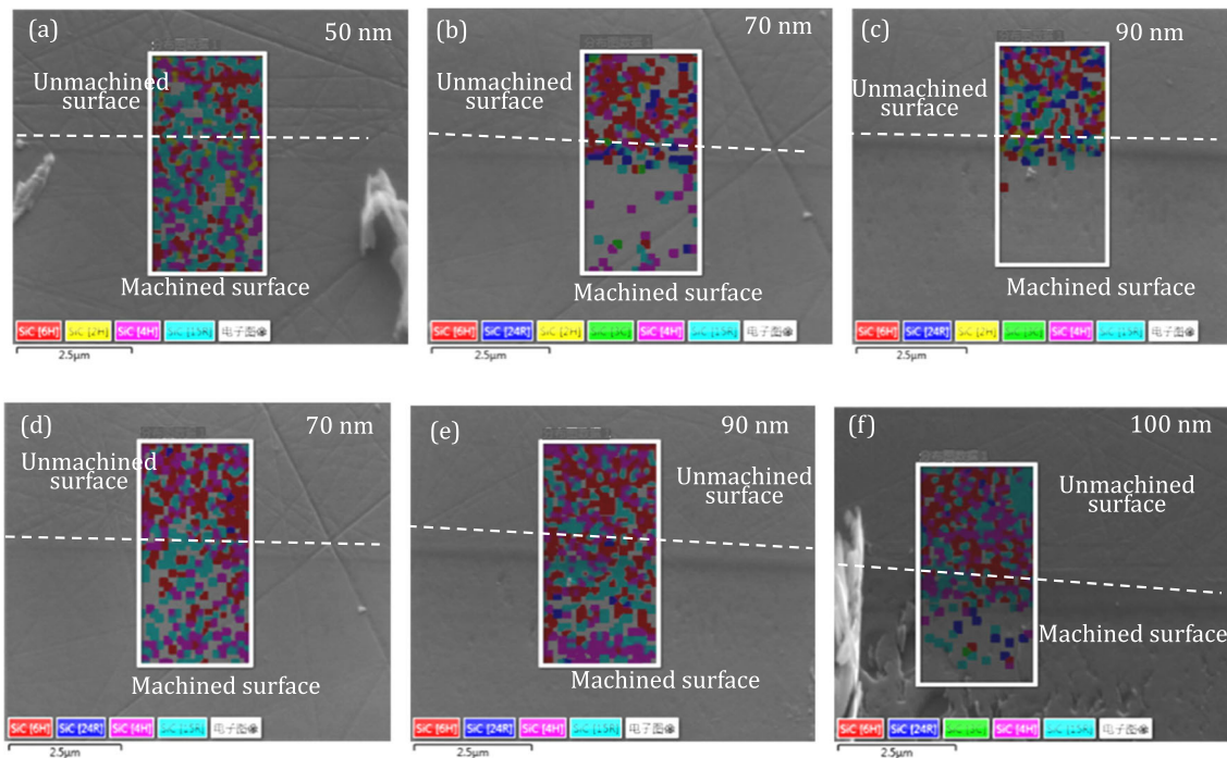
Fig. 4 EBSD images of phase identification and distribution of 6H-SiC after nanocutting. a, b, c are EBSD results under 15 kV and 2.2 nA for undeformed chip thicknesses of 50 nm, 70 nm, and 90 nm, respectively. d, e, f are the EBSD results under 20 kV and 2.4 nA for undeformed chip
