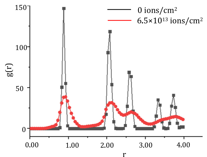
Fig. 13 RDF of the subsurface after ion implantation
