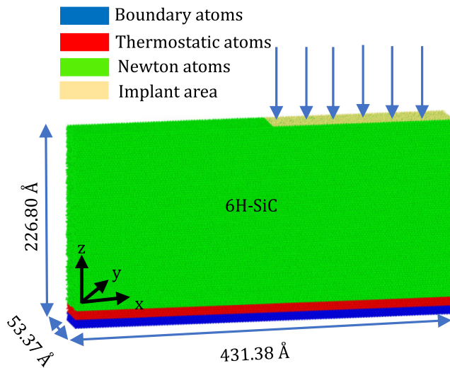
Fig. 10 The implantation MD simulation model
