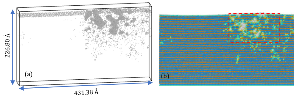
Fig. 11 Damage distribution after ion implantation
