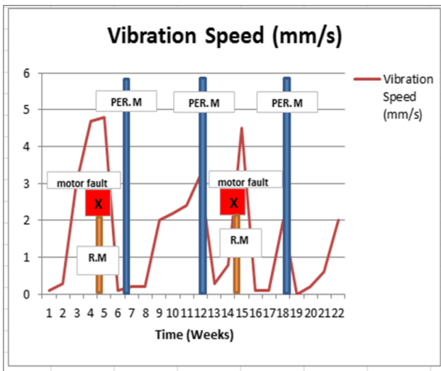
Fig. 22 Motor vibration speed in a system without predictive maintenance
