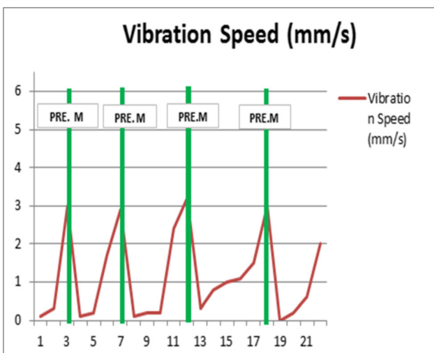
Fig. 23 Motor vibration speed in a system with our predictive maintenance schedule
