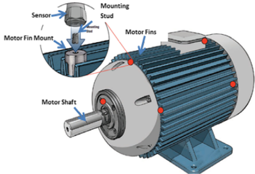
Fig. 5 Vibration sensor mounted on motor— https://www.imi-sensors.com/ContentImages/downloads/IMI-App-Motors_LowRes.pdf
