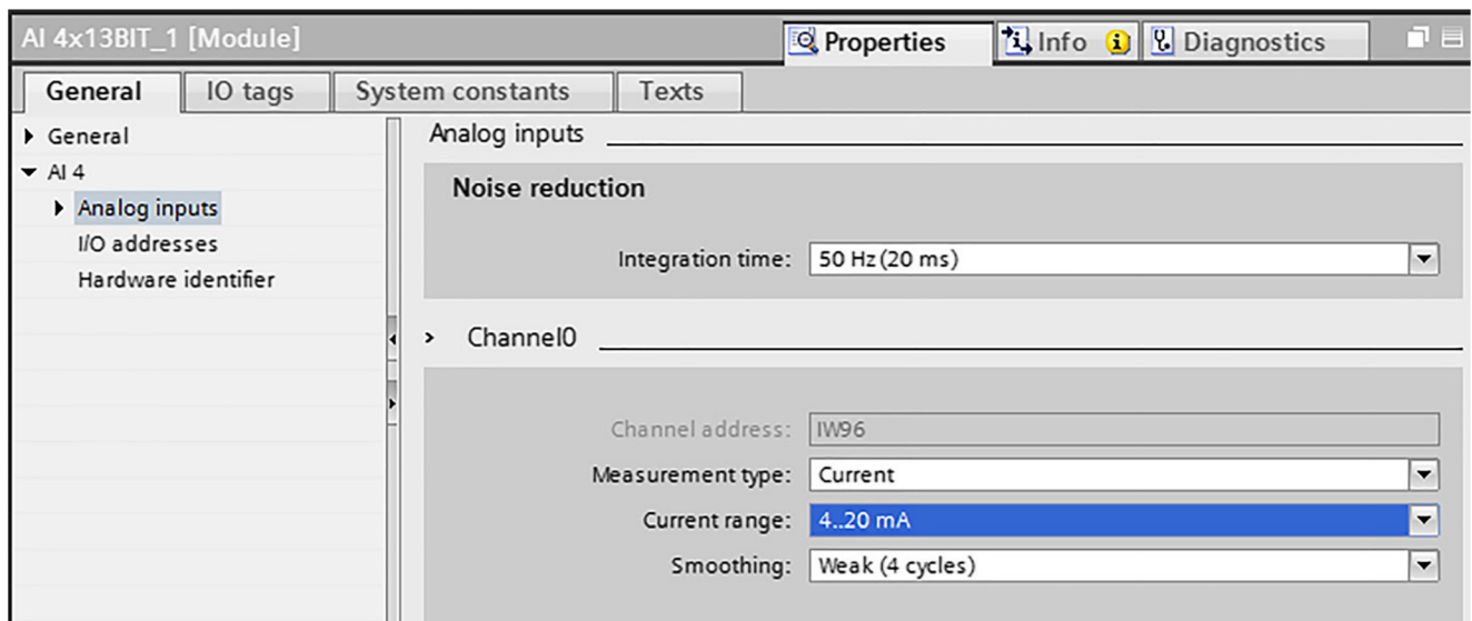
Fig. 28 Analogue input configuration in PLC hardware configuration
