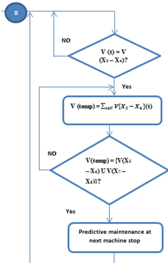
Fig. 8 Predictive maintenance rule flow chart part 3
