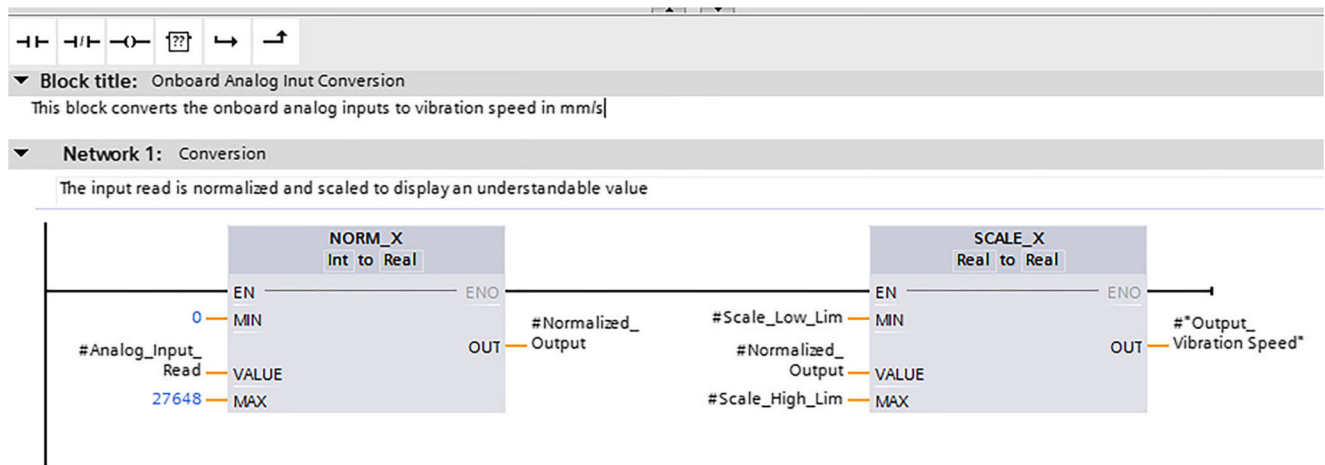
Fig. 29 Analogue input conversion to a real value
