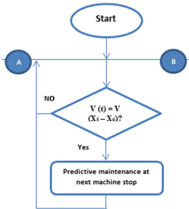
Fig. 7 Predictive maintenance rule flow chart part 2
