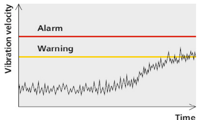
Fig. 3 Machine vibration trend according to ISO 10816—from process monitoring to vibration analysis—www.ifm.com/gb/octavis
