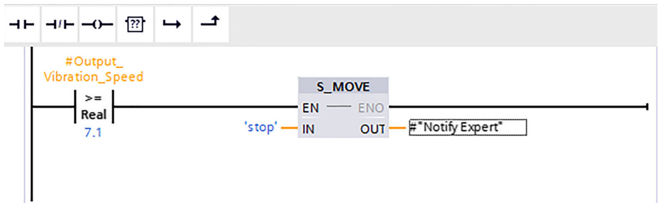
Fig. 30 Vibration speed unacceptable range detection
