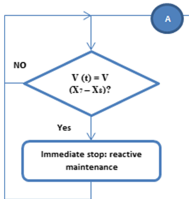
Fig. 6 Predictive maintenance rule flow chart part 1
