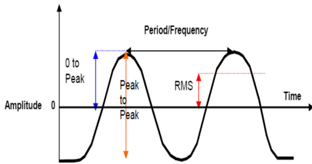
Fig. 1 Vibration as a sine wave—Colin Sanders, “A Guide to Vibration Analysis and Associated Techniques in Condition Monitoring”, DAK Consulting
