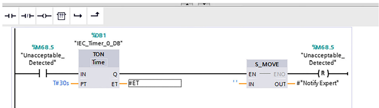
Fig. 31 Reset expert notification variable
