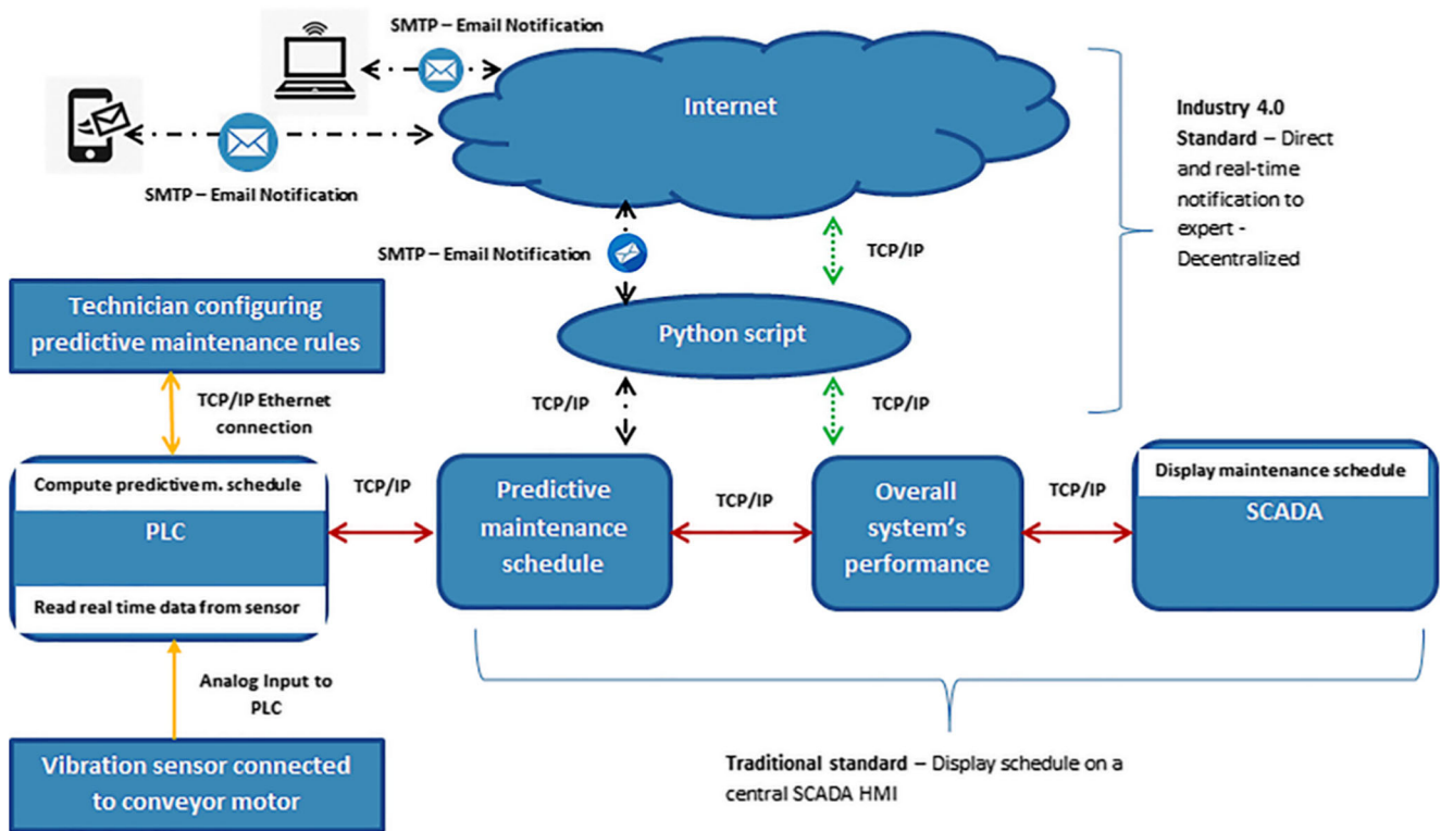
Fig. 25 Overall system's architecture
