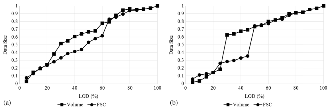
Fig. 7 Decrease in data size during simplification. a Hydrophore. b Horizontal pump model
