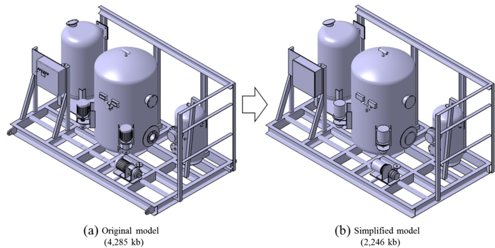
Fig. 8 Final simplification result of the fresh water unit model
