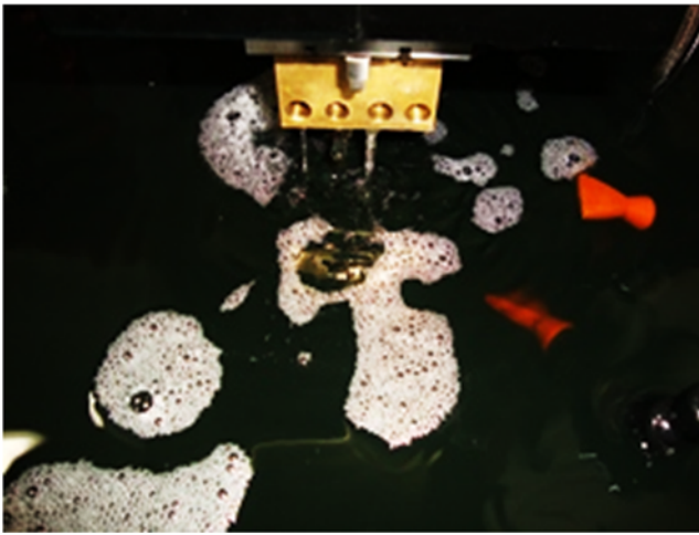
Fig. 4 Mix of kerosene and MWCNTs in the dielectric used for the experiments
