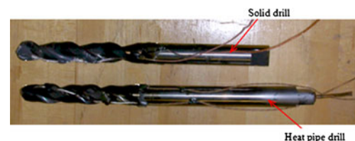
Fig. 4 Solid drill and heat pipe drill
