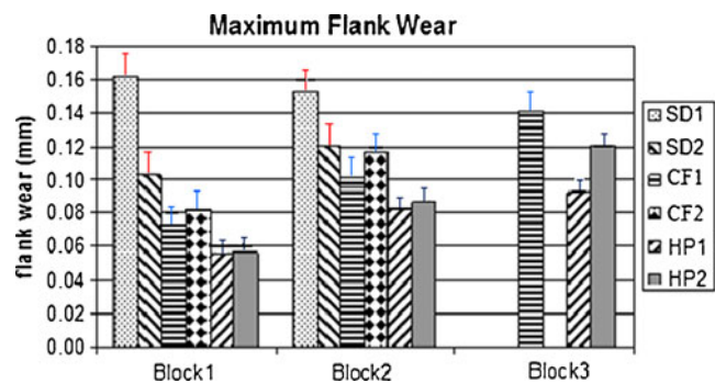
Fig. 12 Maximum flank wear after each block of drilling
