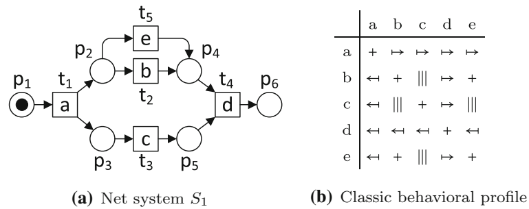
Fig. 1. A net system (a) and its classic behavioral profile (b)
