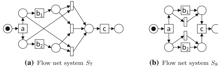
Fig. 7. Two flow net systems that have equal causal behavioral profiles
