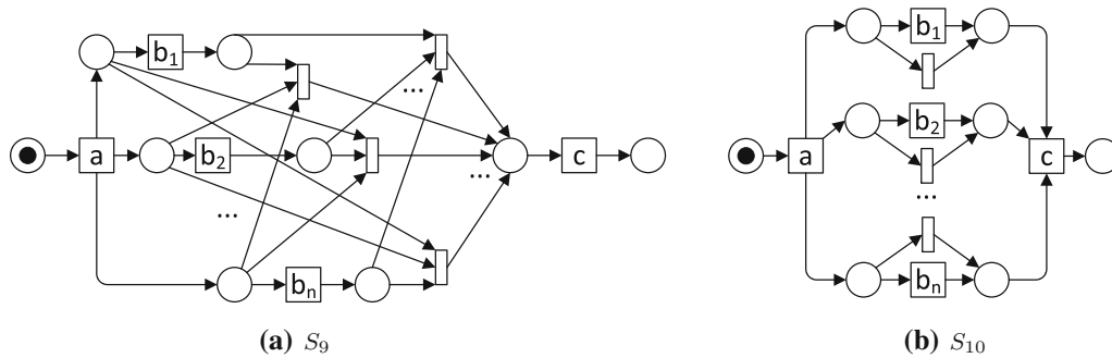
Fig. 8. Generalization of the net systems in Fig. 7
