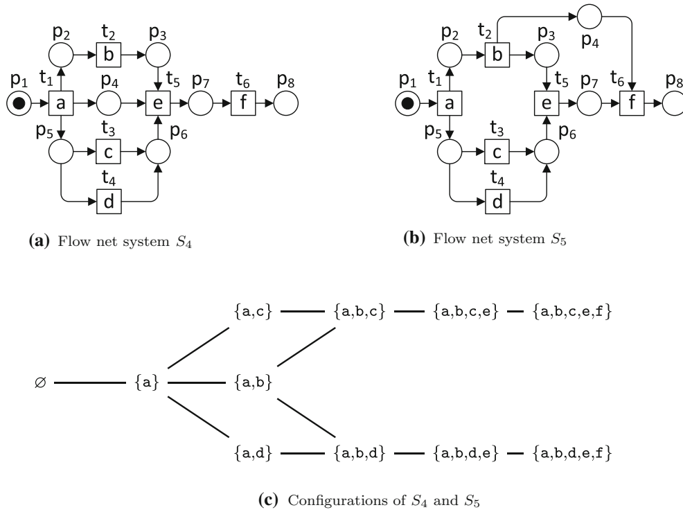
Fig. 3. Flow net systems and their configurations ordered by set inclusion
