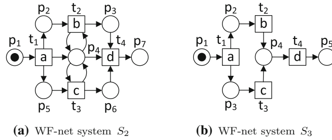
Fig. 2. WF-net systems
