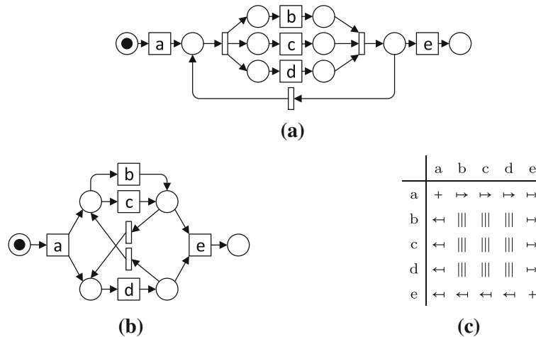
Fig. 9. Two net systems (a, b), and their classic behavioral profile (c)
