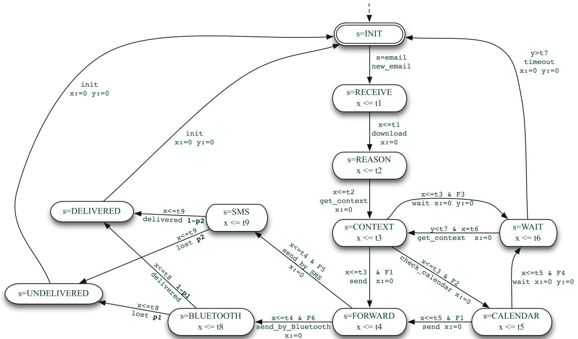
Fig. 7. Scatterbox model
