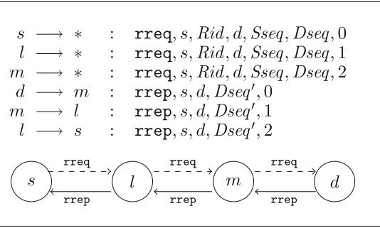
Fig. 1. The AODV routing protocol
