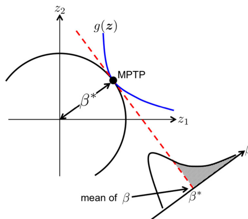
Fig. 4 MPTP search in Z-space
