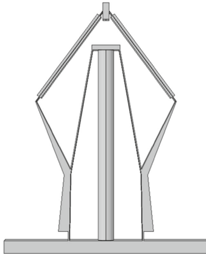
Fig. 17 Optimal configuration of the DMS (proposed method)
