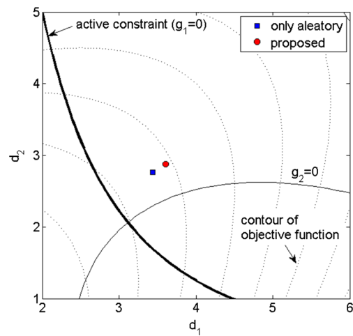
Fig. 13 Optimal solution comparing with and without epistemic uncertainty in example 2
