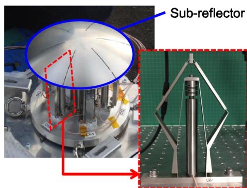
Fig. 20 BBM (breadboard model) of a reconfigurable reflector in the past study (Kogiso et al. 2017)
