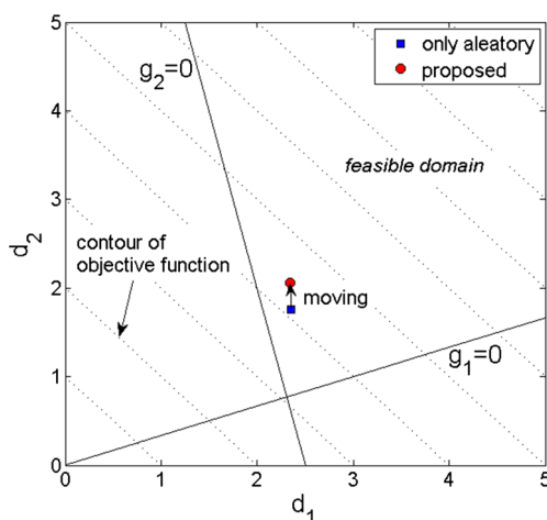
Fig. 11 Optimal solution comparing with and without epistemic uncertainty in example 1
