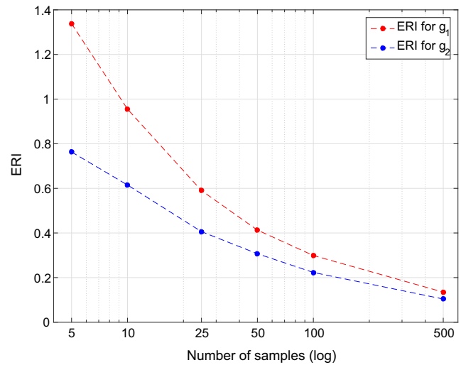
Fig. 23 Relationship between the number of samples and ERI
