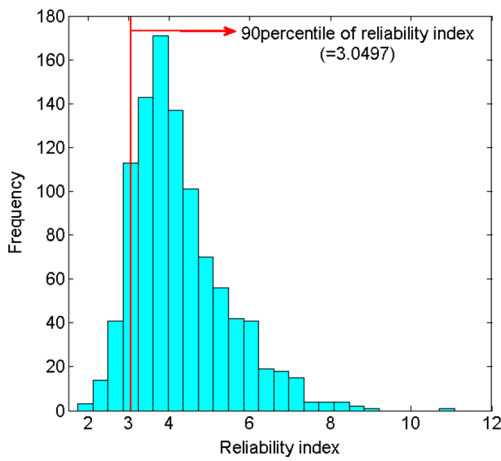
Fig. 14 Validation of the optimal result considering epistemic uncertainty in example 2: histograms of reliability index using MCS sampling
