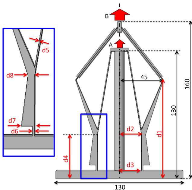
Fig. 15 Displacement magnifying structure
