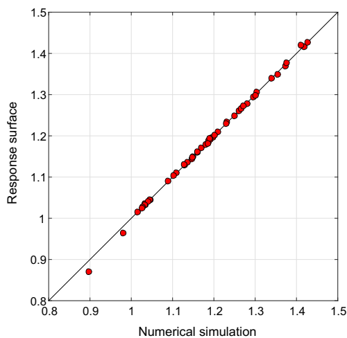
Fig. 22 Accuracy of the response surface of objective function
