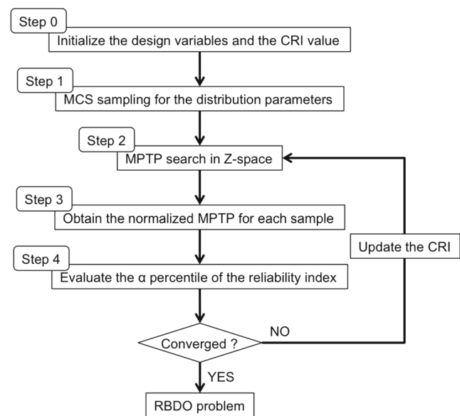
Fig. 6 Procedure of evaluating CRI
