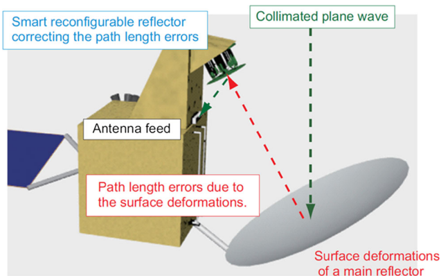
Fig. 19 Smart reflector system (Tanaka et al. 2016)
