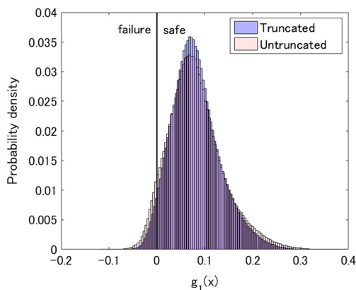
Fig. 16 Result of reliability analysis comparing truncated and untruncated normal distribution
