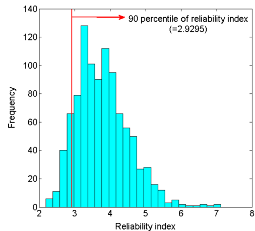
(b) Histogram of reliability index for g_2
