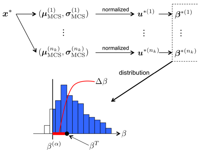
Fig. 5 Evaluating the distribution of the reliability index
