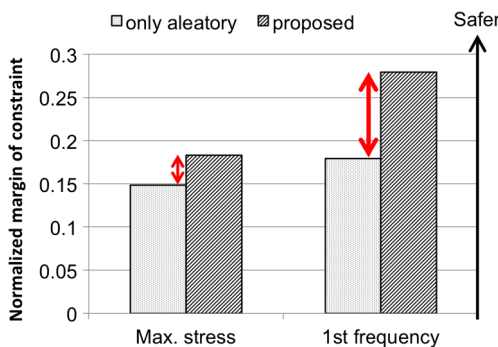
Fig. 18 Comparison of normalized margin of constraint function
