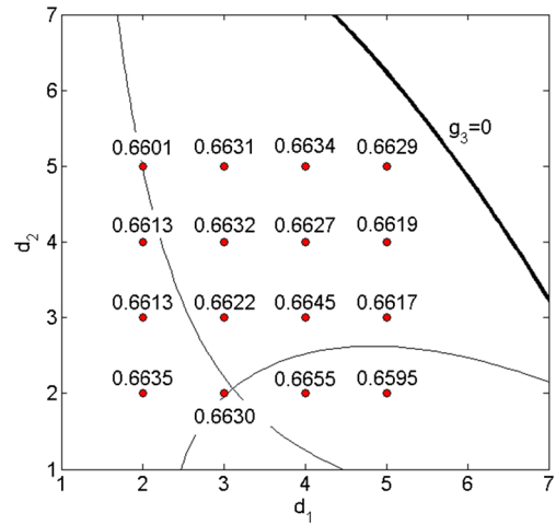
Fig. 10 ERI value of g_3
