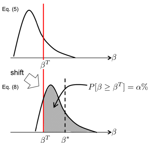
Fig. 3 Shifted reliability index distribution due to conservative target reliability index
