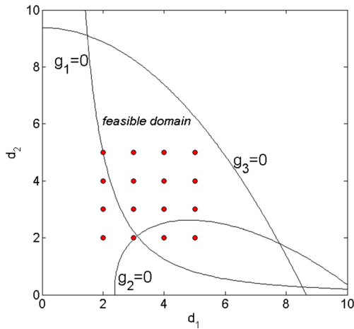
Fig. 7 Grids of the design variable points
