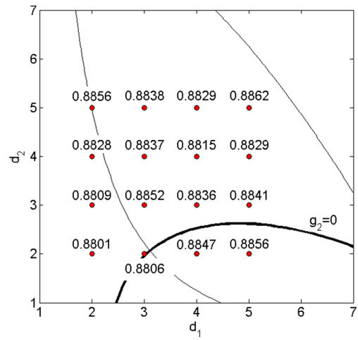
Fig. 9 ERI value of g_2
