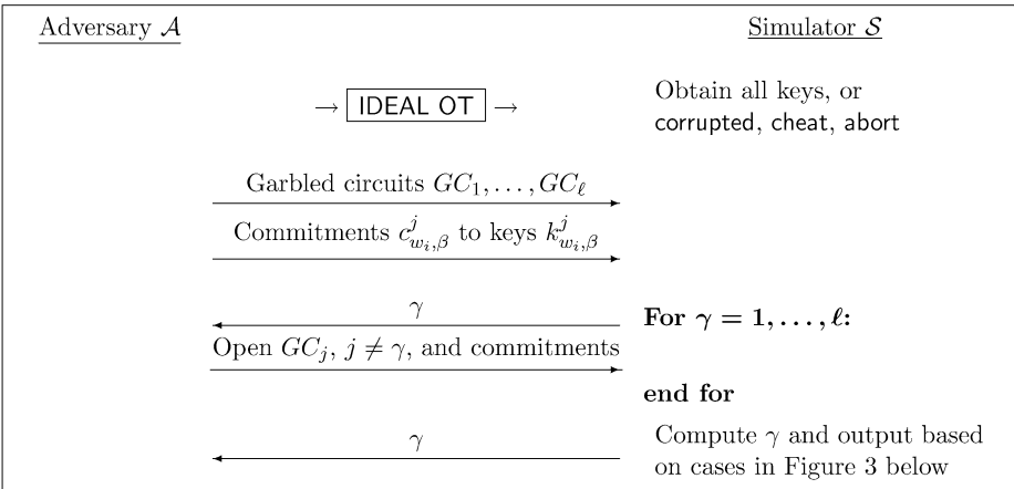
Fig. 2. A high-level diagram of the simulator ( P_1 corrupted).
