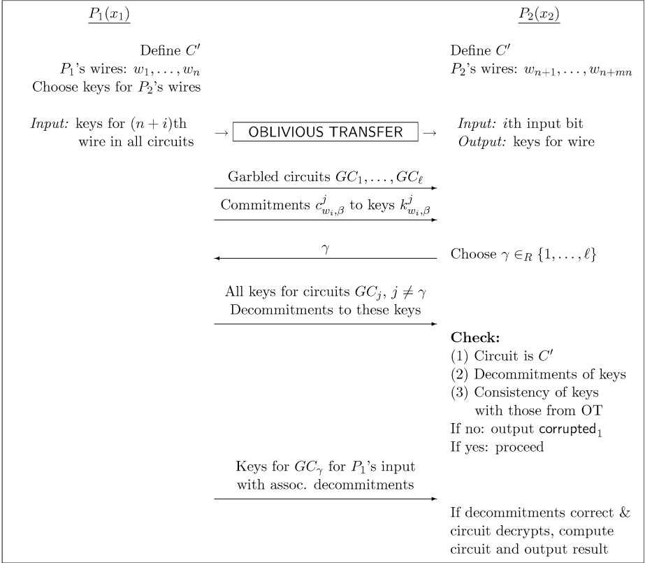
Fig. 1. A high-level diagram of the protocol.
