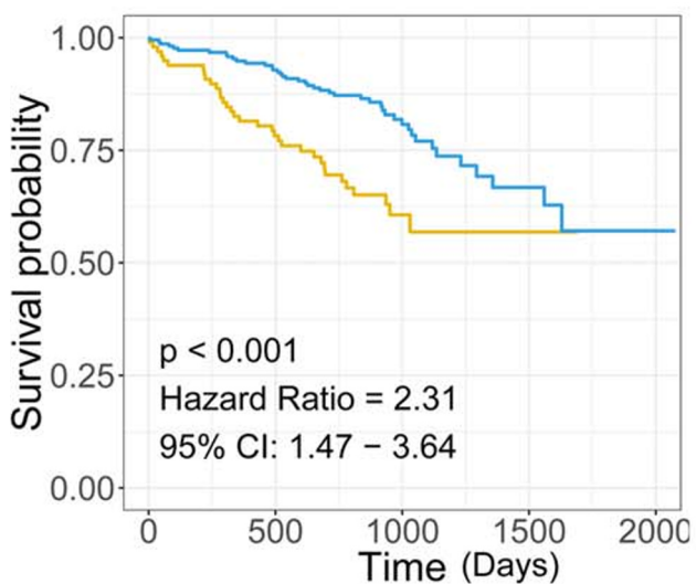
e GSE72094 — High Risk — Low Risk
