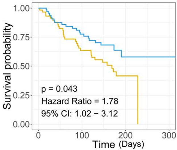
e GSE72094 — High Risk — Low Risk
