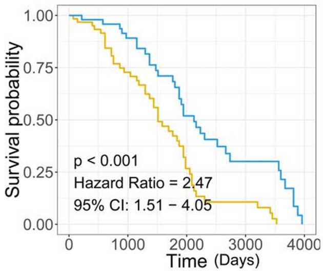
c GSE50081 — High Risk — Low Risk
