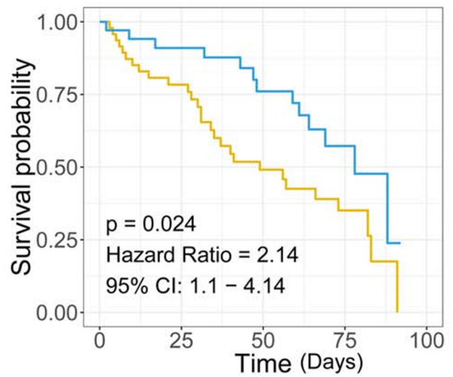
d GSE29013 — High Risk — Low Risk
