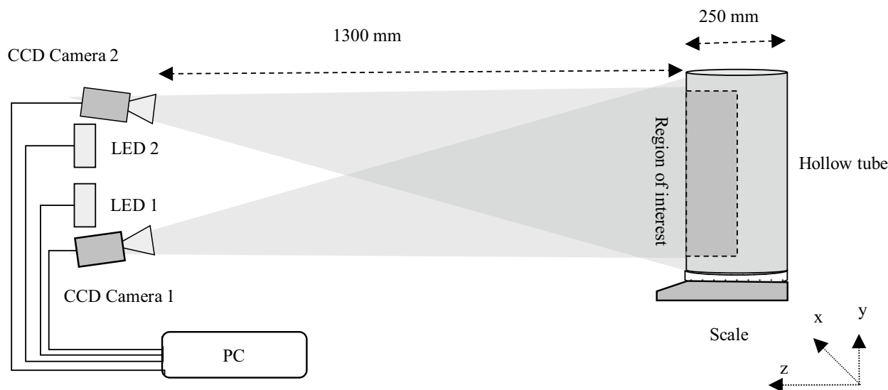
Fig. 3 Schematic of the experimental setup. CCD cameras 1 and 2 were inclined 9° and 25° respectively towards the hollow tube. The region of interest dimension was 400 mm × 250 mm in y and z directions (plane measured)
