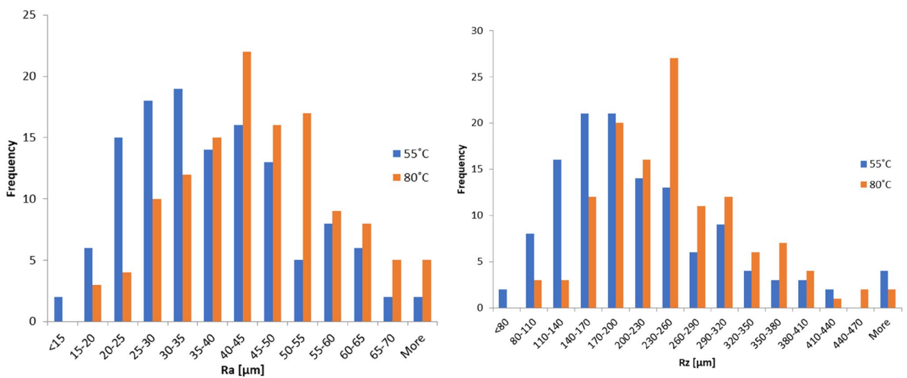
Fig. 8 Distribution of the results of roughness parameters depending on the soaking temperature
