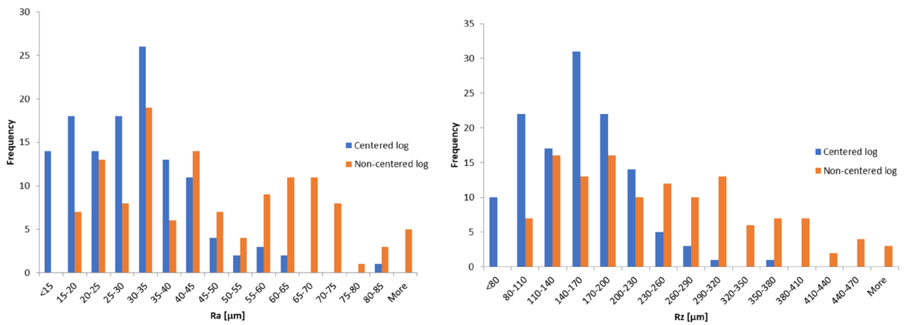
Fig. 7 Distribution of the results of roughness parameters for centered and non-centered logs
