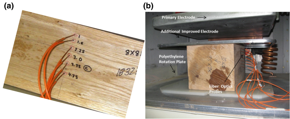
Fig. 2 a Positioning of fiber optic probes in 20 × 20 cm 2 specimen; b RF Heating trial for 25 × 25 cm 2 wood specimen
