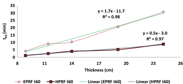
Fig. 4 Relationship between thickness and treatment time [ t_{60} ] for EPRF (3.3–3.4 kW) and HPRF (9.2–10.8 kW)
