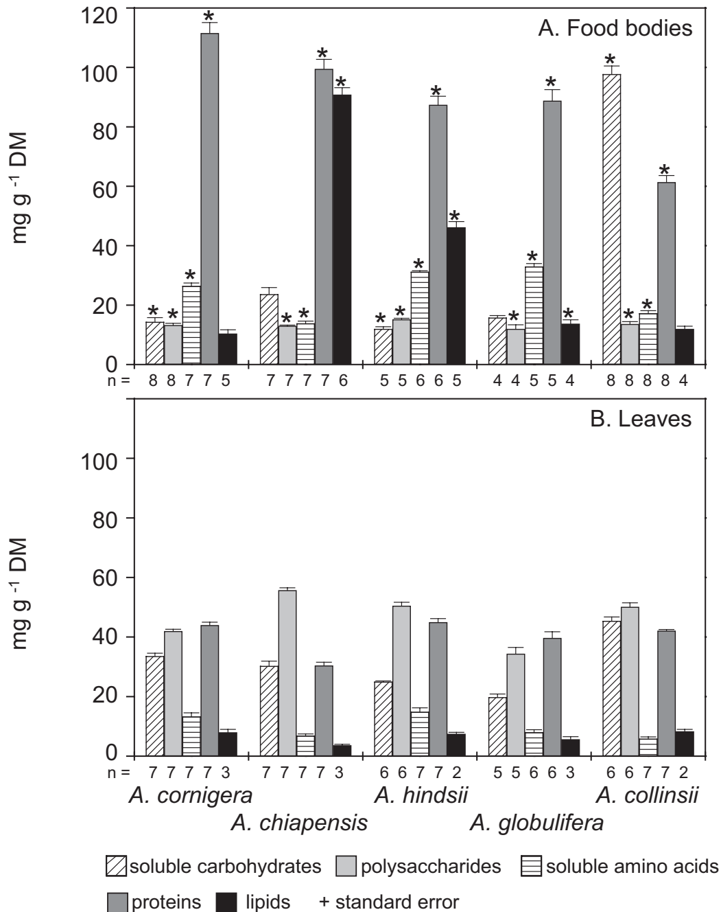
Fig. 3 Contents of main nutrient classes in food bodies (A) and leaves (B) of five myrmecophytic Acacia species. Values are given in \text{mg g}^{-1} dry mass. Sample numbers appear below the bars. Asterisks (*) indicate that contents of individual substance classes differ significantly ( p < 0.05 according to t-test) between food bodies and leaves of the same species
