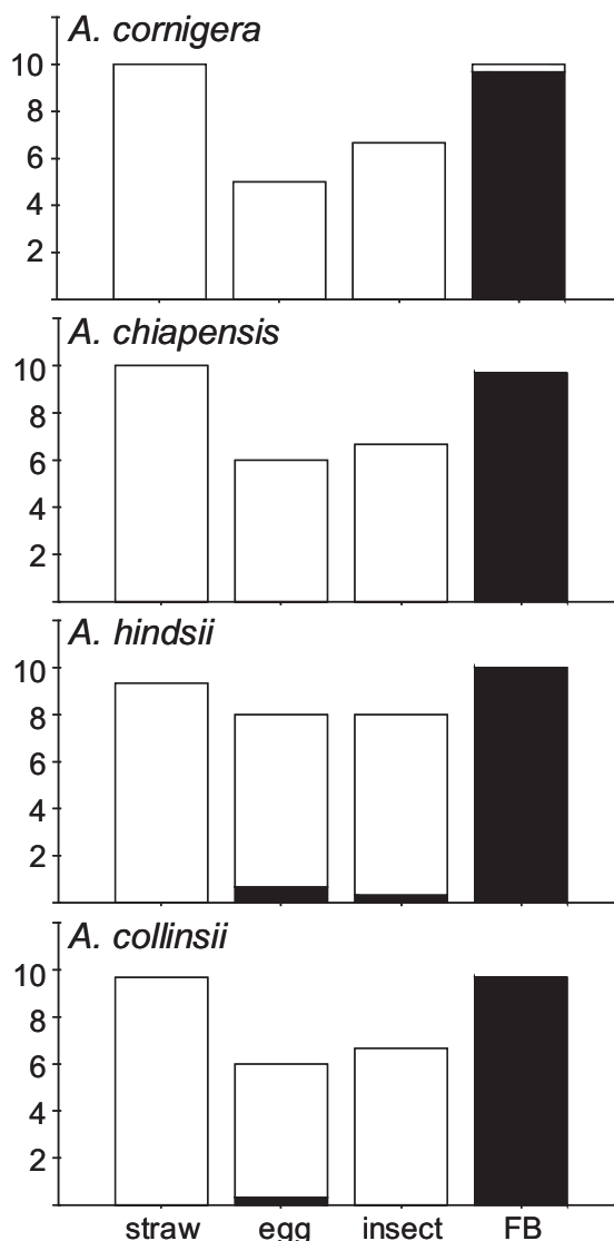
Fig. 2 Behavioural responses of Pseudomyrmex ants to different items offered as putative external food sources. The average number of items offered ( n = 10 per material type and ant colony) that were removed (□) or accepted (■) by the three ant colonies tested per plant species are given separately for the four Acacia species
