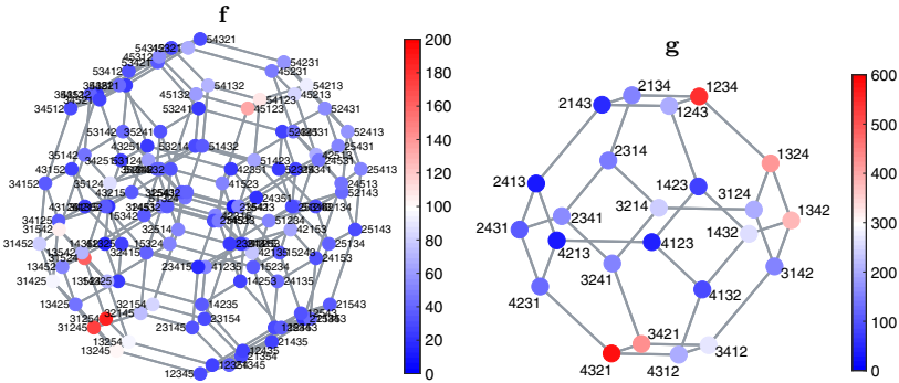
Fig. 1 Left: The signal f on \mathbb{P}_5 represents the vote tallies of 5738 complete rankings of five candidates for APA president in 1980. Right: ranked choice voting data g for the 2017 Minneapolis City Council Ward 3 election, which featured four candidates, shown on \mathbb{P}_4
