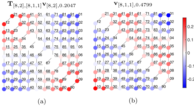
Fig. 23 a The Laplacian eigenvector v_{[8,2],0.2047} , lifted from \mathbb{P}_{[8,2]} to \mathbb{P}_{[8,1,1]} . b The Laplacian eigenvector v_{[8,1,1],0.4799} is orthogonal to the vector in (a) on the Schreier graph \mathbb{P}_{[8,1,1]}
