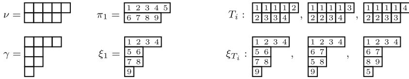
Fig. 30 When v = [5, 4] and \gamma = [4, 2, 2, 1] , the Kostka number is K_{\gamma, v} = 3 . The three column-strict tableaux T_1, T_2, T_3 of shape v and content \gamma are shown here. They each have \gamma_1 = 4 ones, \gamma_2 = 2 twos, \gamma_3 = 2 threes, and \gamma_4 = 1 four. The set partitions \pi_1 \in \Pi_v and \xi_1 \in \Pi_\gamma are in reading order, and \xi_{T_1}, \xi_{T_2}, \xi_{T_3} \subseteq \Pi_\gamma are the set-partitions with T_i fillings; that is \xi_{T_i} has j is row r if the j th box of T_i (read in reading order) contains r
