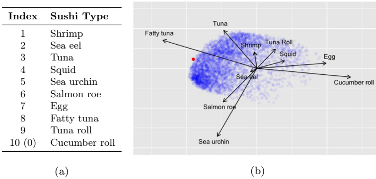
Fig. 2 a Candidate items in the sushi preference data set [50,51]. b Projection of sushi preference signal, h , onto two dimensions using Gabriel’s biplot. Each blue dot represents a single voter (of the 5000 total), and the transparency is indicative of the number of voters, with darker shades indicating a higher density of voters. The poles associated with the popular sushi items tend to fall towards the left on the fatty tuna–cucumber roll axis. The projection of the Condorcet ranking is plotted in red
