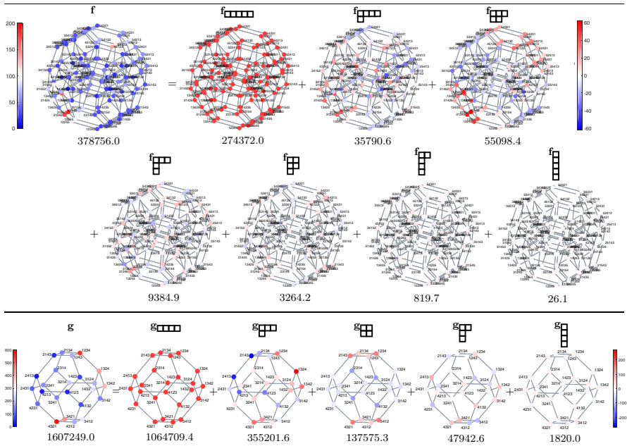
Fig. 3 Decomposition of the signals of Fig. 1 into orthogonal vectors in each of their respective isotypic components. The numbers below the signals show how the energy \|f\|^2 splits into the energies \|f_\gamma\|^2 . The first of these energies is a function of the number of voters (e.g., 274372 = 5738^2/120 for the APA data of [29]). The second is a measure of the first order effect given by the number of voters who rank candidate i in position j . The third and fourth capture the unordered and ordered second order (pair) effects, respectively, net of the first order marginal effects
