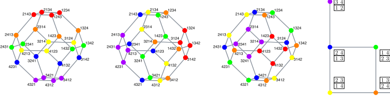
Fig. 13 Right: The Schreier graph \mathbb{P}_{\boxplus} = \mathbb{P}_{[2,2]} (shown without self loops). Recall from Fig. 12 that we view the vertices of the Schreier graph as ordered set partitions of ranking slots . Left: three different equitable partitions of \mathbb{P}_4 that yield this Schreier graph, corresponding to the ordered set partitions \pi_1 = \{\{1, 2\}, \{3, 4\}\} , \pi_2 = \{\{1, 3\}, \{2, 4\}\} , and \pi_3 = \{\{1, 4\}, \{2, 3\}\} , respectively, from left to right. We view the three equitable partitions on the left as set partitions of candidates . For each equitable partition, all vertices of the permutahedron with the same color are mapped to the node of the corresponding color on the Schreier graph; this mapping is encoded in the rows of the characteristic matrix \mathbf{B}_{\pi_i} . For each equitable partition, the two pairs of candidates defined by the ordered set partition \pi_i are in the ranking slots defined by the two rows of the tableaux with the corresponding color in the Schreier graph on the right. For example, in the middle equitable partition \pi_2 , the red vertices correspond to rankings where candidates 1 and 3 are in ranking positions 1 and 2, and candidates 2 and 4 are in positions 3 and 4
