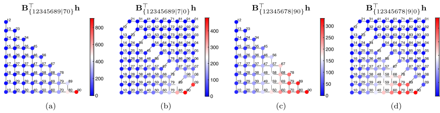
Fig. 24 Projections capturing the second order ordered and unordered marginals for the pairs of sushi items 7/10 and 9/10
