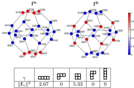
Fig. 6 Two signals on \mathbb{P}_4 with the same energy decomposition into isotypic components; i.e., \|\mathbf{f}^a_\gamma\| = \|\mathbf{f}^b_\gamma\| := \|\mathbf{f}_\gamma\| for all \gamma
