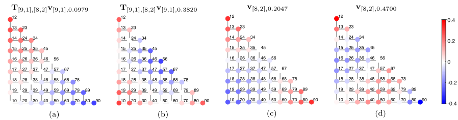
Fig. 22 a and b The Laplacian eigenvectors \mathbf{v}_{[9,1],\lambda} , for \lambda = 0.0979 and \lambda = 0.3820 , lifted from \mathbb{P}_{[9,1]} to \mathbb{P}_{[8,2]} . c and d The Laplacian eigenvectors \mathbf{v}_{[8,2],\lambda} , for \lambda = 0.2047 and \lambda = 0.4700 , are orthogonal to each other and to the two vectors in (a) and (b) on the Schreier graph \mathbb{P}_{[8,2]}
