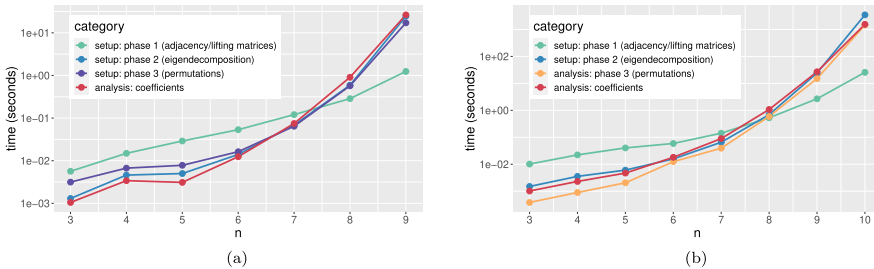
Fig. 32 Computation times for the setup and analysis portions in our a base implementation, and b more memory efficient implementation that moves some of the phase 3 setup computation into the analysis portion of the code
