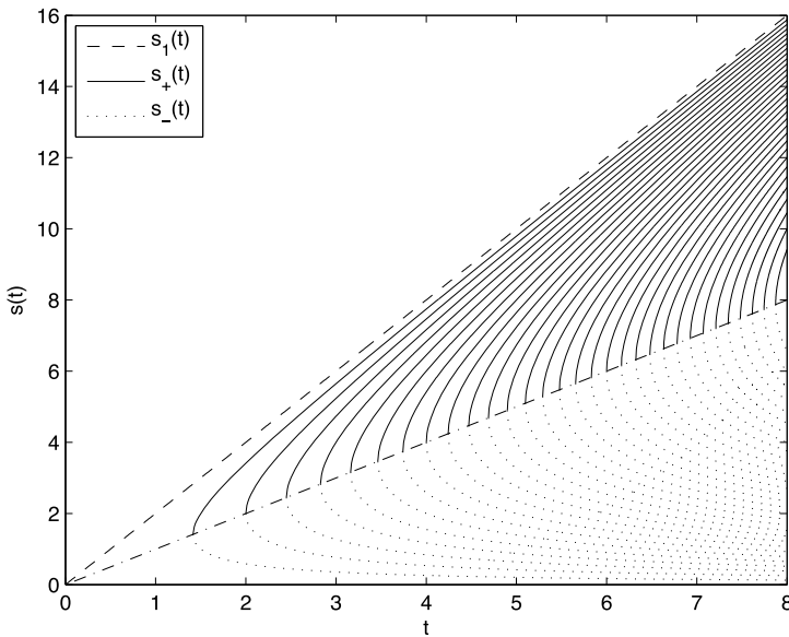
Fig. 1 Solutions (31) of the reassignment equations for positive times. The dashed, full and dotted lines correspond to the solutions referred to respectively as s_1(t) , s_+(t) and s_-(t) in the text, with the Hermite function order increasing from 1 to 33 when going from left to right. The locus of fixed points for the reassignment operators has been superimposed as the dashed-dotted line
