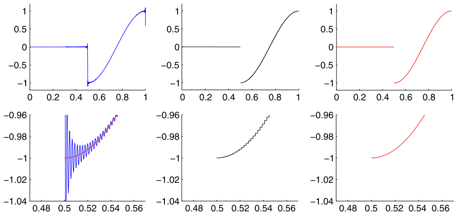
Fig. 7 The upper figures show g_N (left), \tilde{g}_{n,m} (middle) and g (right) on the interval [0, 1] . The lower figures show g_N (left), \tilde{g}_{n,m} (middle) and g (right) on the interval [0.47, 0.57]
