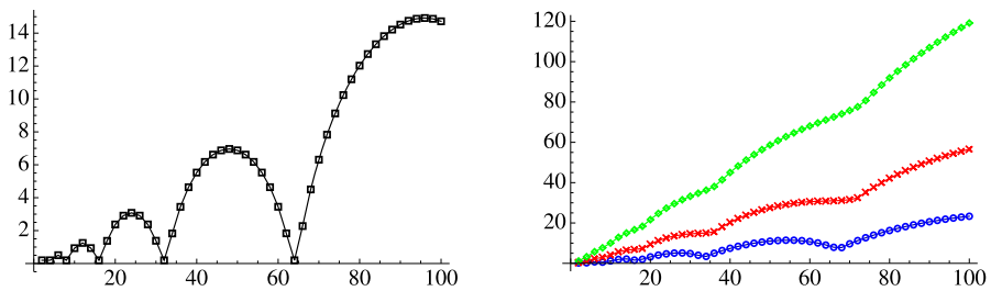
Fig. 2 This figure shows \log_{10} \|(S_{\epsilon,m}^* W_m)^{-1}\| as a function of m and \epsilon for m = 1, 2, \dots, 100 . The left plot corresponds to \epsilon = 1 , whereas the right plot corresponds to \epsilon = 7/8 (circles), \epsilon = 1/2 (crosses) and \epsilon = 1/8 (diamonds)
