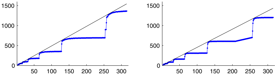
Fig. 5 The figure shows sections of the graphs of \tilde{\Psi}(U, \cdot, 1) (left) and \tilde{\Psi}(U, \cdot, 2) (right) together with the functions (in black) x \mapsto 4.9x (left) and x \mapsto 4.55x . In this case U is formed by using the Haar wavelets on [0, 1]
