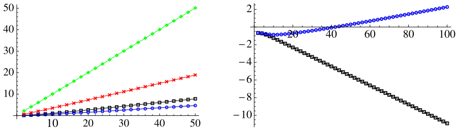
Fig. 3 The left figure shows \log_{10} \|(S_{\epsilon, m}^* W_m)^{-1}\| as a function of m for m = 2, 4, \dots, 50 and \epsilon = 1, \frac{7}{8}, \frac{1}{2}, \frac{1}{8} (squares, circles, crosses and diamonds respectively). The right figure shows \log_{10} \|f - P_{\mathcal{W}_m} f\| (squares) and \log_{10} \|f - \tilde{f}\| (circles) for m = 2, 4, 6, \dots, 100 , where f(x) = \frac{1}{1+16x^2}
