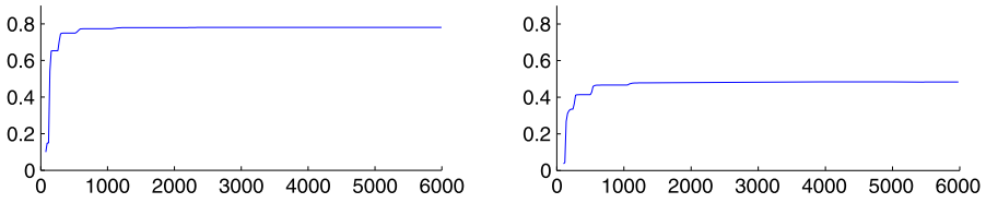
Fig. 4 The figure shows K_{n,m,M} for n = 75, m = 350 and M = n + 1, \dots, 6000 (left) and K_{n,m,M} for n = 100, m = 400 and M = n + 1, \dots, 6000 (right) for the Haar wavelets on [0, 1]
