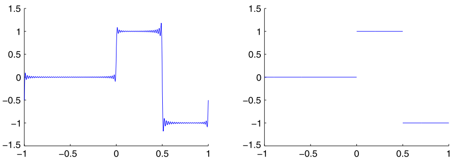
Fig. 1 The figure shows \Lambda_{N,\epsilon,2}(f) for f = \mathcal{F}g , N = 500 and \epsilon = 0.5 (left) as well as g (right)
