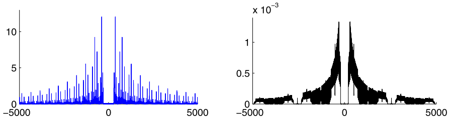
Fig. 9 The figure shows the error |f - f_N| (left) and |f - \tilde{f}| (right) on the interval [-5000, 5000]
