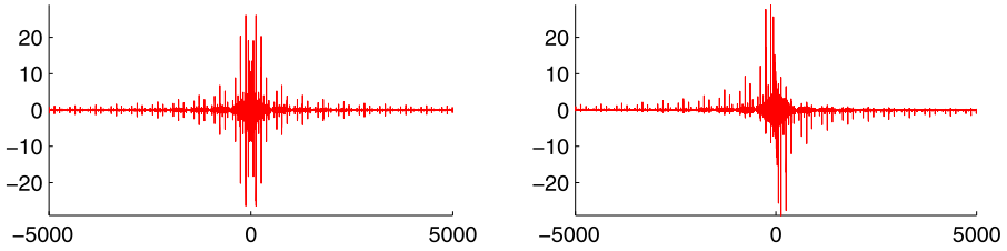
Fig. 8 The figure shows \text{Re}(f) (left) and \text{Im}(f) (right) on the interval [-5000, 5000]
