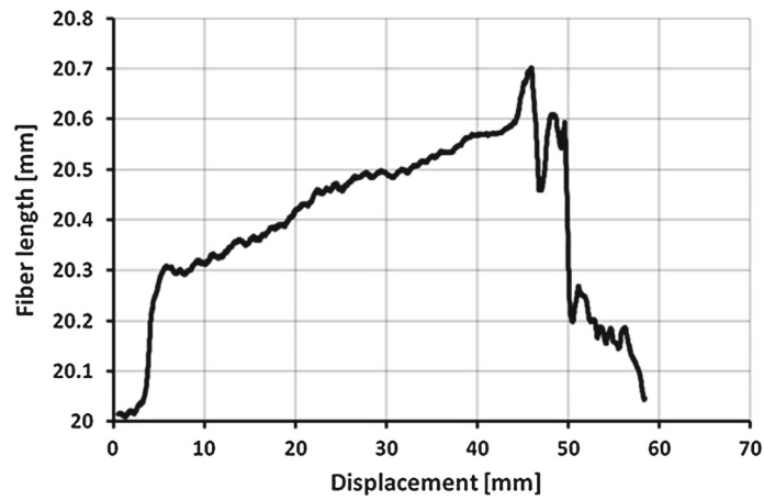
FIG. 16. Fiber length versus displacement curve registered during tensile test of sample 3
