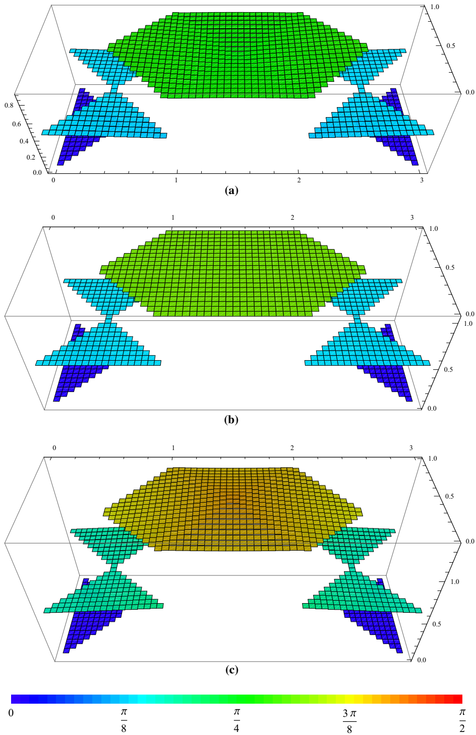
FIG. 5. Total angle \vartheta_1 + \vartheta_2 for several values of imposed relative displacement when W_1^I is used: a u_x = u_y = 0.65 * L , b u_x = u_y = (\sqrt{3} - 1) * L , c u_x = u_y = 0.8 * L
