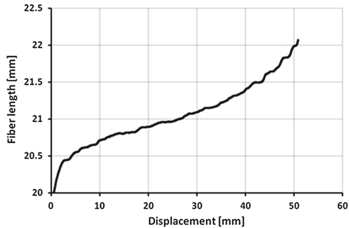
FIG. 14. Fiber length versus displacement curve registered during tensile test of sample 1
