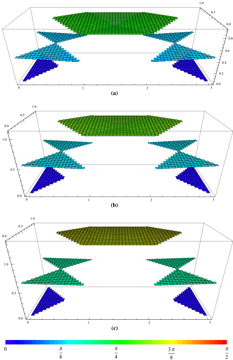
FIG. 6. Total angle \vartheta_1 + \vartheta_2 for several values of imposed relative displacement when W_2^I is used: a u_x = u_y = 0.65 * L , b u_x = u_y = (\sqrt{3} - 1) * L , c u_x = u_y = 0.8 * L
