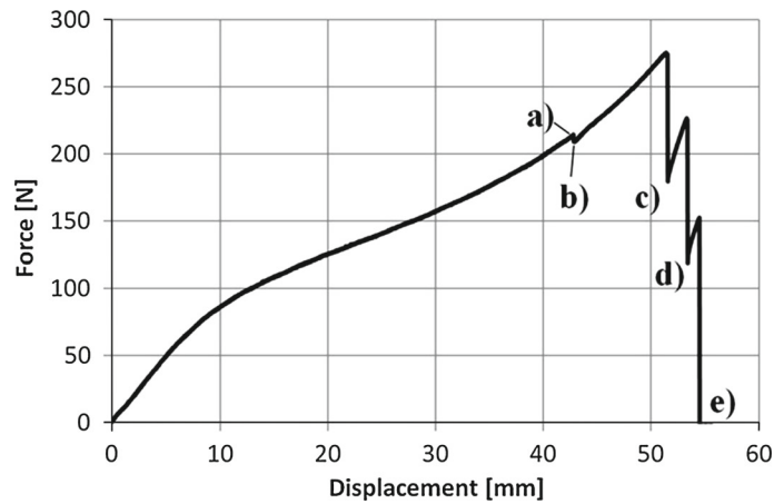
FIG. 20. Force versus displacement curve registered during tensile test of sample 1 with characteristic points corresponding to pictures in Fig. 17
