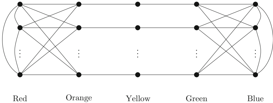
Fig. 2 The FI-graph of Example 3.16. The key feature is that there are n ‘bridges’ from the right side of the graph to the left, and any Hamiltonian path must cross each of them
