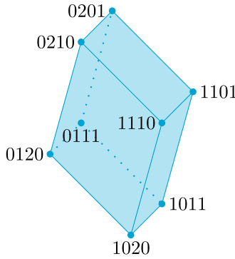
FIGURE 2. The graphic zonotope Z_{\text{Path}_4} is a parallelepiped
