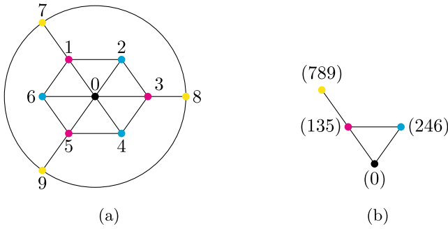
FIGURE 4. A graph \Gamma with the orbits of its vertices under the automorphism \sigma = (0)(135)(246)(789) colored (a), and the corresponding graph C_\Gamma(\sigma) (b)
