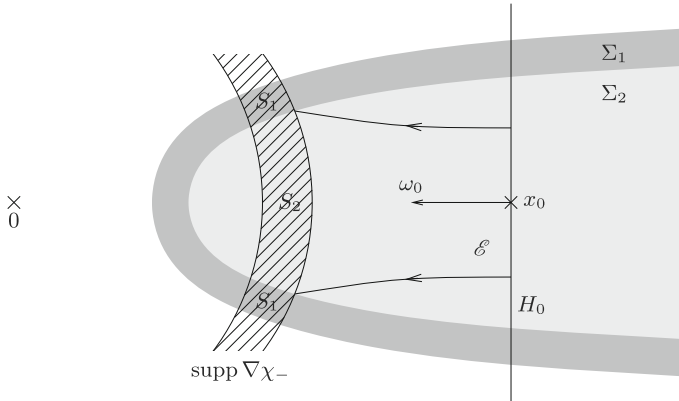
FIGURE 12. Geometric setting in the proof of Theorem 5.6
