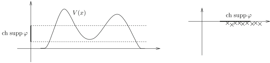
FIGURE 4. Geometric setting and the resonances of Q in Example 3.7
