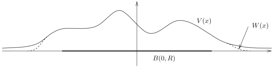
FIGURE 1. Potentials V and W given by (A2)
