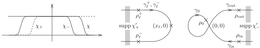
FIGURE 8. Cut-off functions \chi_\star and the geometry of Corollary 4.7
