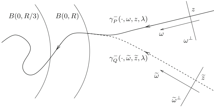
FIGURE 11. Canonical relation \Lambda_{Q \leftarrow P}^{\text{ini}}
