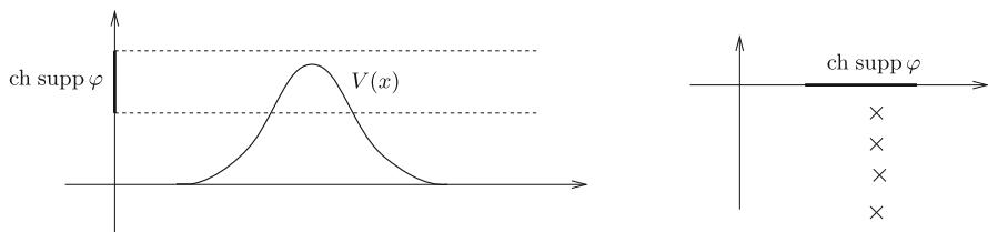
FIGURE 5. Geometric setting and the resonances of Q in Example 3.9
