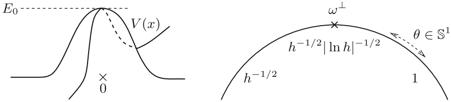
FIGURE 9. Potential of Example 5.1 and the order of the scattering amplitude in function of the final direction \theta \in \mathbb{S}^1
