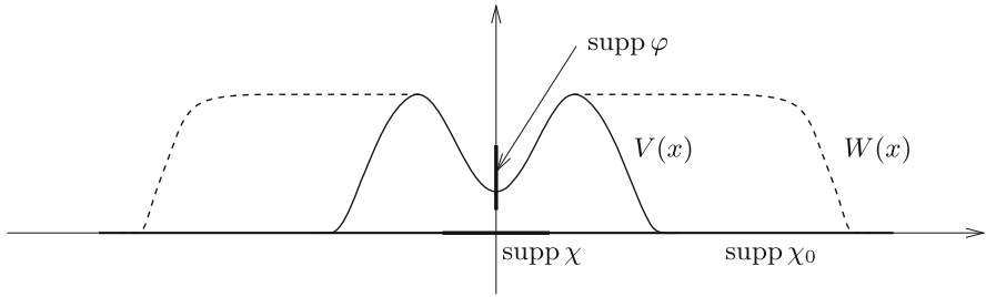
FIGURE 3. Setting in the proof of Remark 3.4
