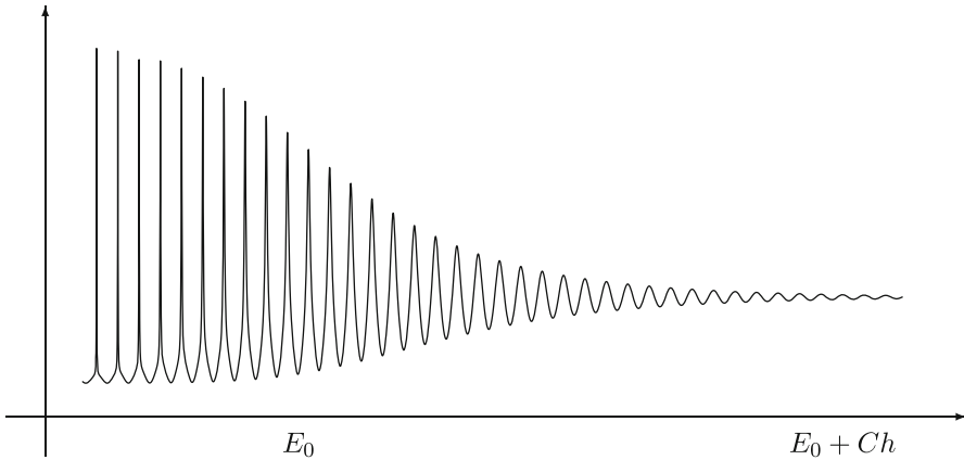
FIGURE 7. Derivative of the SSF given by Corollary 4.7
