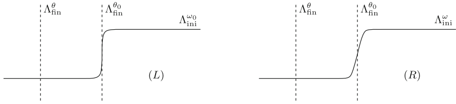
FIGURE 10. A cross section of the Lagrangian manifolds \Lambda^\star
