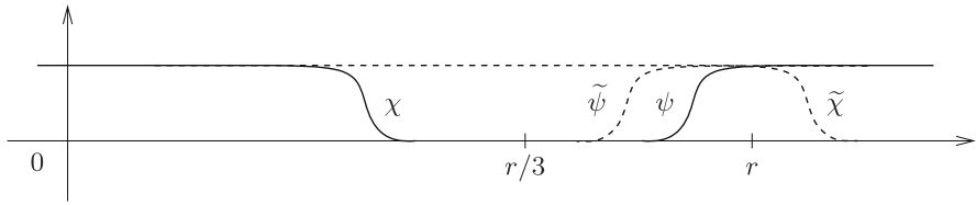
FIGURE 13. Various functions in the proof of Theorem 2.1
