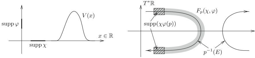
FIGURE 2. On the left, an example of potential V in dimension n = 1 . On the right, the associated set F_p(\chi, \varphi) and the energy surface p^{-1}(E) for some E \in \text{supp } \varphi
