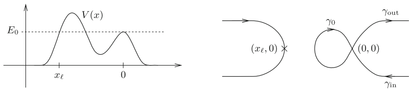
FIGURE 6. Geometric setting of Example 4.6
