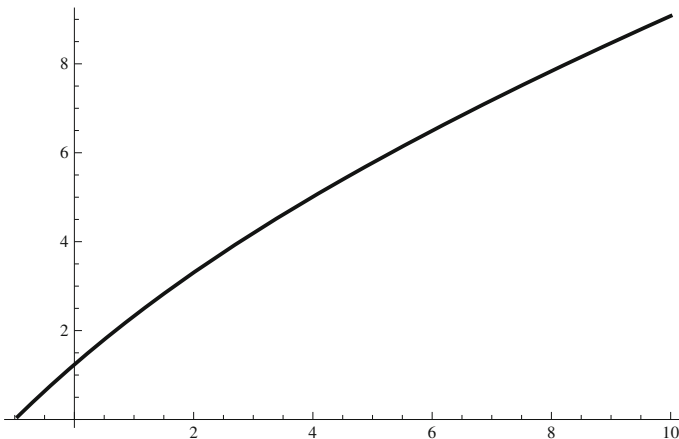
FIGURE 1. Case d = 2, p = 3, B = 1 : plot of \alpha \mapsto (2\pi)^{2/p-1} \mu_{\mathbf{B}}(\alpha)
