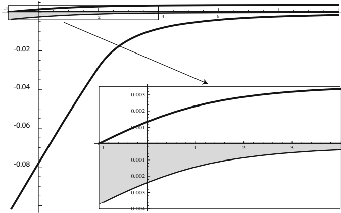
FIGURE 2. Case d = 2, p = 3, B = 1 : comparison of the upper estimates \alpha \mapsto \mu_{\text{Gauss}}(\alpha) and \alpha \mapsto \mu_{\text{EL}}(\alpha) of Sects. 5.1 and 5.2, with the lower estimates \alpha \mapsto \mu_{\text{interp}}(\alpha) and \alpha \mapsto \mu_{\text{LT}}(\alpha) of Propositions 3.1 and 4.2. Plots represent the curves \log_{10}(\mu_{\text{Gauss}}/\mu_{\text{EL}}) , \log_{10}(\mu_{\text{LT}}/\mu_{\text{EL}}) and \log_{10}(\mu_{\text{interp}}/\mu_{\text{EL}}) so that \alpha \mapsto \mu_{\text{EL}}(\alpha) corresponds to a straight line at level 0. The exact value associated with \mu_{\mathbf{B}} lies in the gray area
