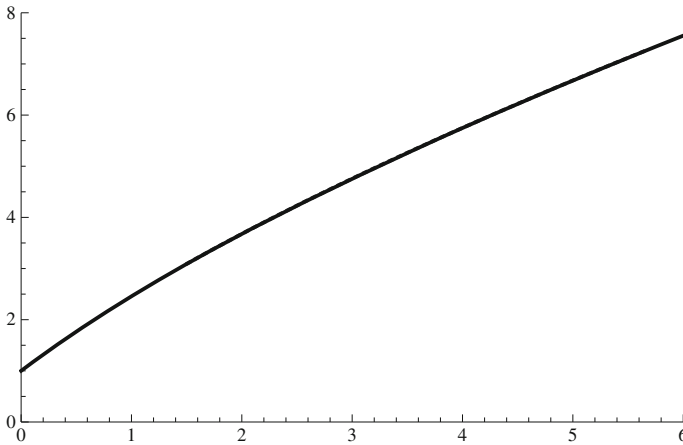
FIGURE 3. Case d = 2, p = 1.4, B = 1 : plot of \beta \mapsto \nu_{\mathbf{B}}(\beta) . The horizontal axis is measured in units of (2\pi)^{1-2/p} \beta
