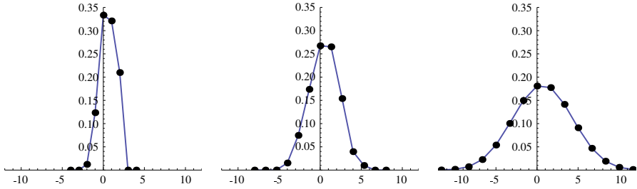
FIGURE 1. An O.Q.R.W. on \mathbb{Z} which gives rise to a centered Gaussian at the limit, while starting clearly uncentered (at times n = 4, n = 8, n = 20 )
