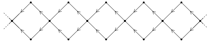
FIGURE 1. Example of an admissible, non-injective directed graph.
