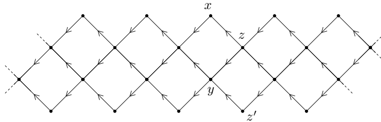
FIGURE 3. Example of an admissible, injective directed graph.
