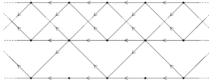
FIGURE 7. Example of an admissible, non-injective directed graph.
