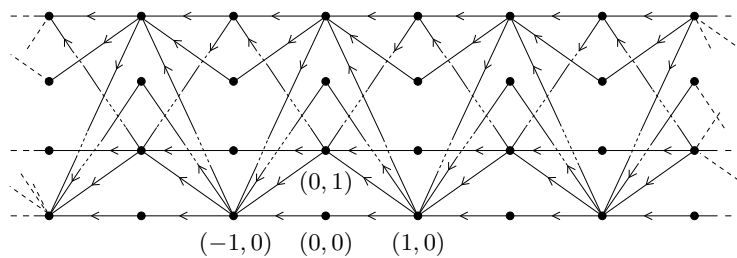
FIGURE 4. Example of an admissible directed graph.
