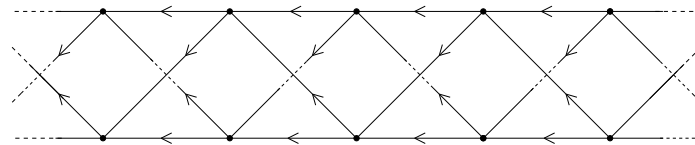
FIGURE 6. Example of an admissible, non-injective directed graph.
