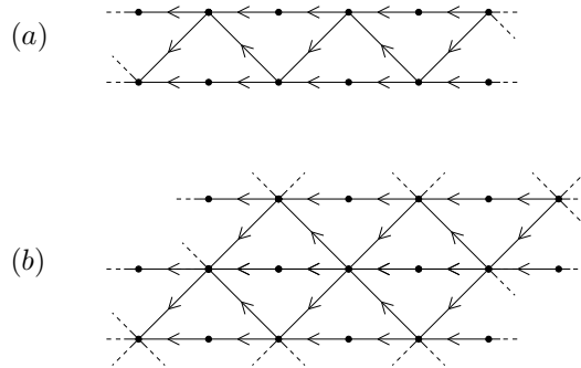
FIGURE 5. Examples of admissible, injective directed graphs.
