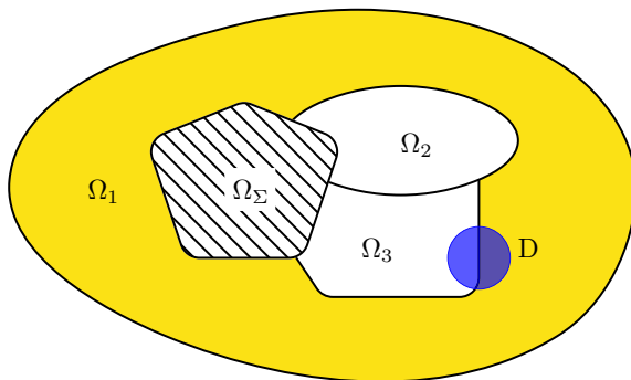
FIGURE 2. Geometrical situation for part ③ of the proof of Lemma 4.5. Here j = 1 , \overline{\mathcal{O}}_1 = \overline{\Omega}_\Sigma \cup \overline{\Omega}_2 \cup \overline{\Omega}_3 and \ell = 3
