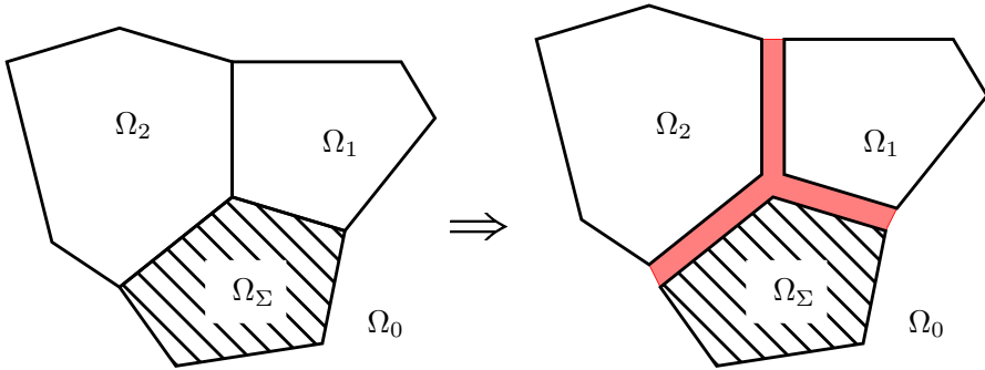
FIGURE 5. Illustration of the gap idea (gap highlighted)
