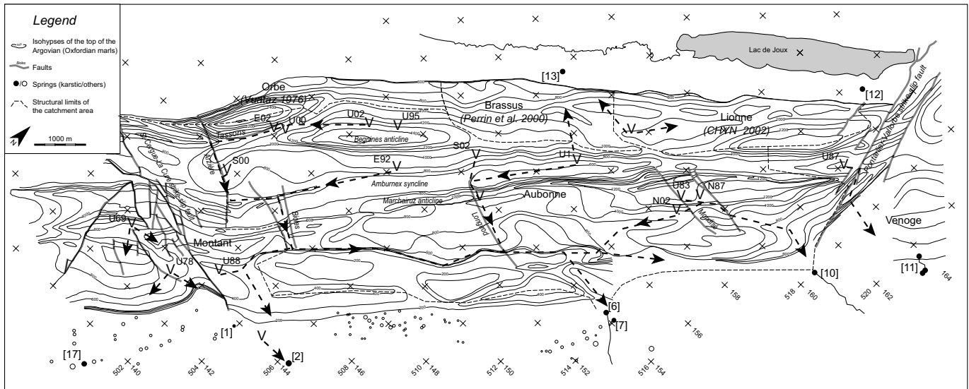
Fig. 7. Structural map of the top of the Oxfordian marls (adapted after Aubert et al. 1979, Falconnier 1951 and Lagotla 1920) and proposed limits of the catchment area of the Aubonne spring. This catchment area, based on structural criteria, is in good agreement with measured water balance and tracing experiments. Results of the tracer tests allow a first schematization of the main flow routes.
