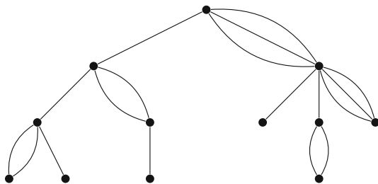
FIGURE 1. A 5-ary multi-edge tree
