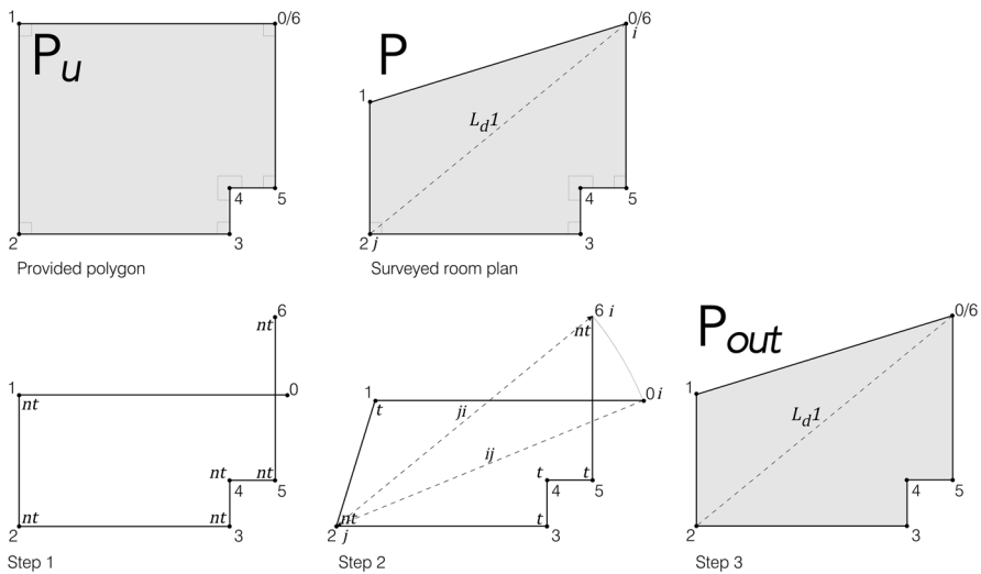
Fig. 6 An example of triangulation of a polygon terminating with Pattern00 algorithm
