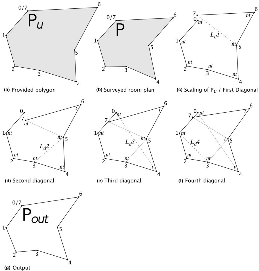
Fig. 10 Case Study 3: triangulation of a room starting with a user-provided polygon with no orthogonal corners
