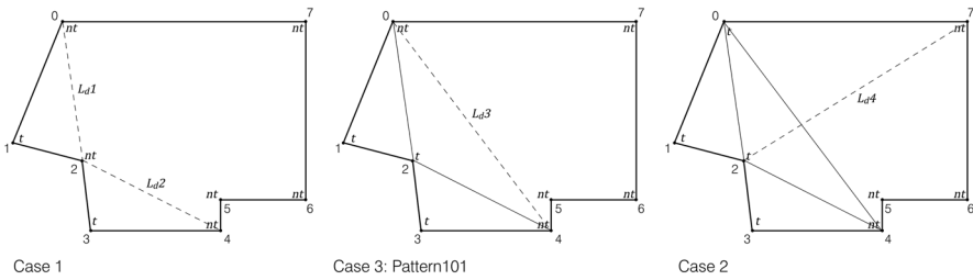
Fig. 4 An example of a possible triangulation sequence using each of the described triangulation cases
