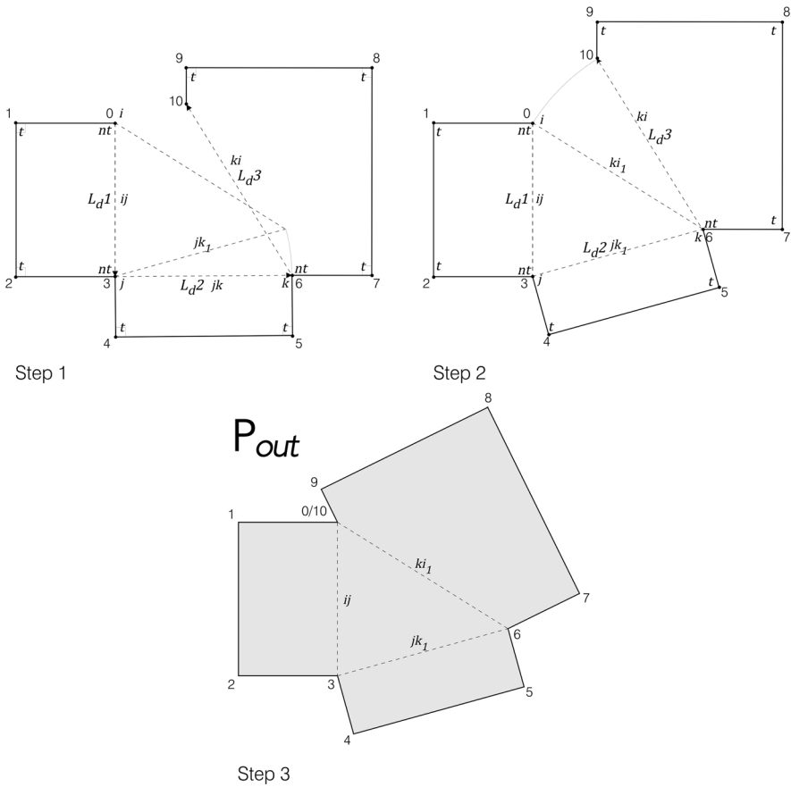
Fig. 7 Application of the algorithm Pattern000. t is a corner that can be triangulated by a diagonal
