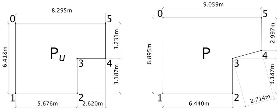
Fig. 2 P is the actual plan of the room, and P_u is a polygon with arbitrary side lengths and a similar morphology to P
