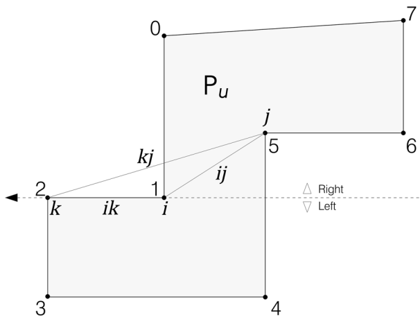
Fig. 5 An example of a j on the right of the infinite line from i to k in the triangulation of the ij chain
