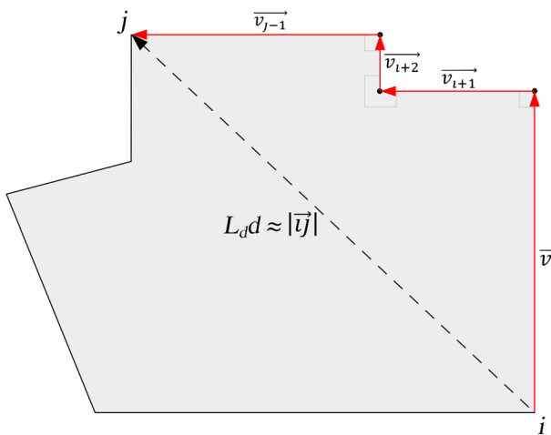
Fig. 3 Example of polygonal chain closure on the ij chain
