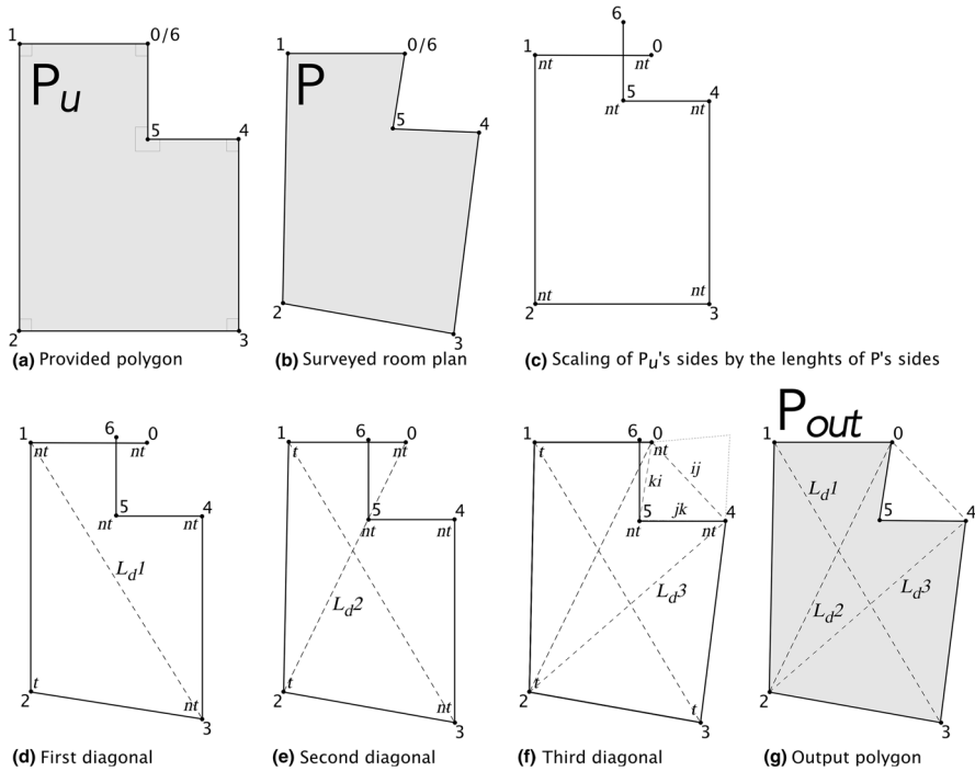
Fig. 8 Case Study 1: triangulation of a polygon terminating with Pattern000 algorithm
