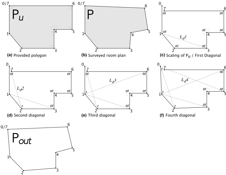
Fig. 9 Case Study 2: triangulation of a room starting with a user-provided polygon with some non-orthogonal corners
