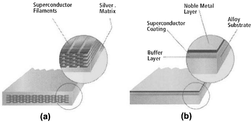
Fig. 11.24 Superconducting metal matrix composites: (a) first generation high temperature superconductor (HTS) filaments in a silver matrix ( in commercial production), (b) second generation coated conductor composite, consisting of a superconductor layer, coated with a noble metal, on an alloy substrate (courtesy of J. Jackson, American Superconductor).
