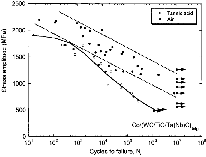
Fig. 8.19 S-N curve for WC/Co composites in air and in tannic acid at 4 Hz (after Pugley and Sockel, 2004). The effect of corrosion fatigue effect, at low stress amplitudes, is clear.
