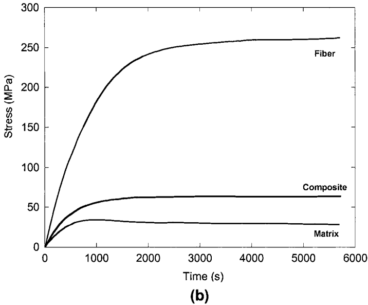
Fig. 9.4 Evolution of load transfer during creep, from the creeping matrix to the rigid reinforcement: (a) schematic of experimental behavior and (b) three-dimensional finite element model (after Sørensen et al., 1992). As the matrix creeps, an increased fraction of the load is transferred to the fibers. Upon unloading, slight creep recovery in the matrix takes place.
