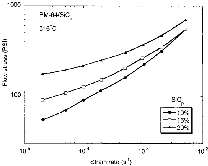
Fig. 9.20 Slow stress versus strain rate during superplasticity at 516°C of an Al alloy matrix composites reinforced with SiC particles (after Mahoney and Ghosh, 1987). An increase in SiC volume fraction resulted in an increase in the flow stress necessary for superplasticity.
