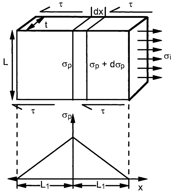
Fig. 7.5 Schematic of modified shear lag analysis used to quantify load transfer in low aspect ratio particles (after Nardone and Prew, 1986).
