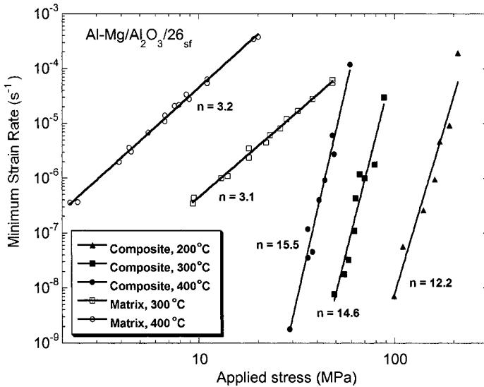
Fig. 9.14 Comparison of creep behavior of Al-5Mg/Al 2 O 3 /26 sf versus the unreinforced alloy (after Dragone and Nix, 1992). Anomalously high values of the stress exponent, n, were observed in the composite.
