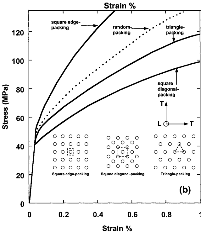
Fig. 7.23 Finite element model predictions of tensile behavior of continuous fiber reinforced composites with varying fiber arrangement (after Brockenbrough et al., 1991): (a) longitudinal and (b) transverse.
