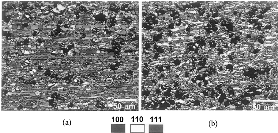
Fig. 4.31 Orientation imaging map of matrix grains in a 2080/SiC p composite: (a) parallel to extrusion axis and (b) perpendicular to extrusion axis. The matrix exhibits a [100]\langle 111 \rangle texture, typical of deformation processed FCC materials. Perpendicular to the extrusion direction, the texture is random, indicating an overall fibrous texture.
