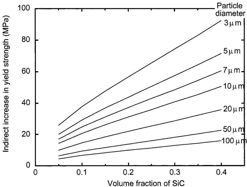
Fig. 7.9 Increase in yield strength due to dislocation punching, as predicted by the model of Arsenault and Shi (1986). The degree of strengthening is significantly influenced by particle size, for a given volume fraction.
