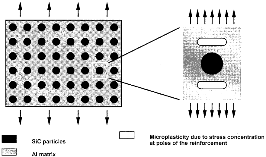
Fig. 7.25 Microplasticity in the matrix of particle reinforced MMCs due to stress concentrations at the poles of the reinforcement and/or at sharp corners of the reinforcing particles (after Chawla et al., 1998b).
