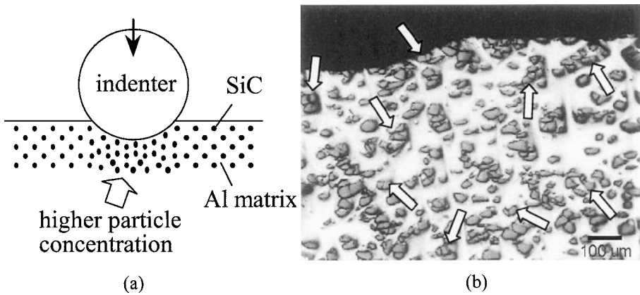
Fig. 7.43 Deformation behavior of particle reinforced MMCs during microindentation (after Shen and Chawla, 2001): (a) localized increase in particle concentration due to plastic flow of the matrix and (b) localized particle fracture, indicated by the arrows.
