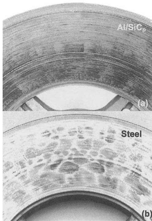
Fig. 11.19 Thermal cracking behavior in (a) Al/SiC p and (b) steel after wear testing (courtesy of H. Ruppert). The steel brake shows significant amount of cracking (white lines) while the MMC is in relatively good condition.
