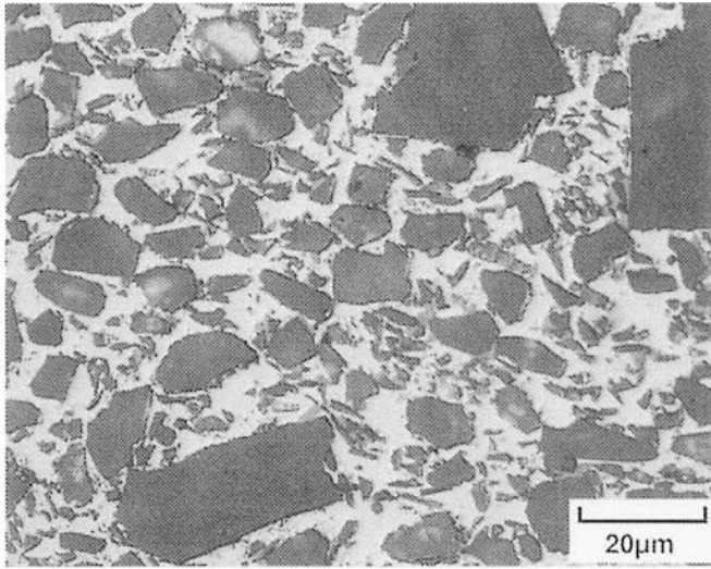
Fig. 11.21 Microstructure of SiC particle reinforced Al matrix composite used for thermal applications (courtesy of M. Occhionero, Ceramic Process Systems). The bimodal particle size distribution enables a large volume fraction of particles ( > 50\% ) to be used.
